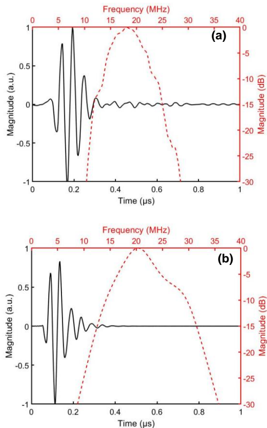
Fig. 7. (a) Normalized measured (element #75) and (b) simulated pulse echo response (black, solid lines) of one representative array element and its corresponding frequency responses (red, dashed lines).
