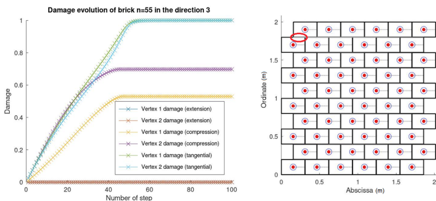
Fig. 13.6: Evolution of damage with respect to iterations in a specific part of the masonry.
