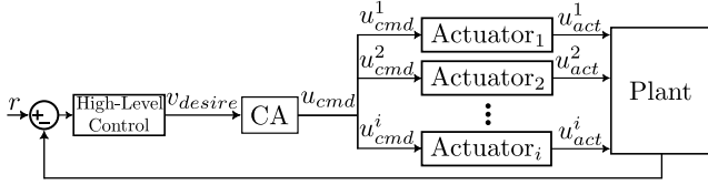
Fig. 1. Control allocation problem scheme.
