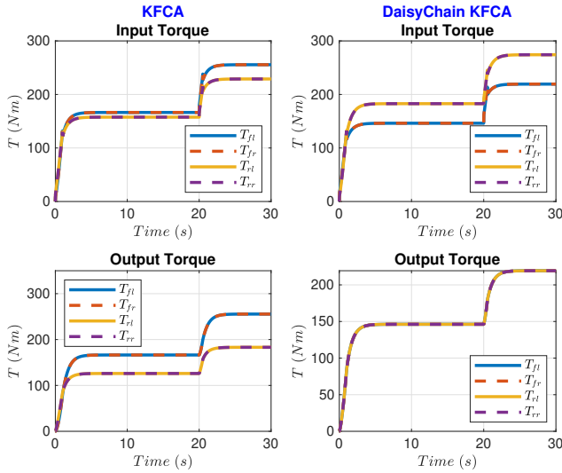
Fig. 2. Actuator Inputs/Outputs in Scenario 1.
