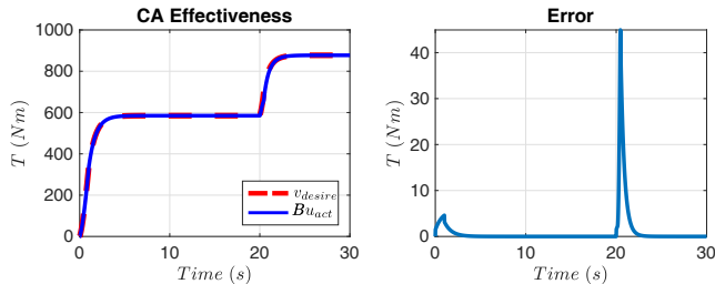
Fig. 3. Total torque commanded and its relative error in Scenario 2.
