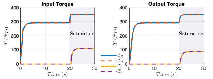
Fig. 4. Actuator Inputs/Outputs using DCKFCA in Scenario 2.
