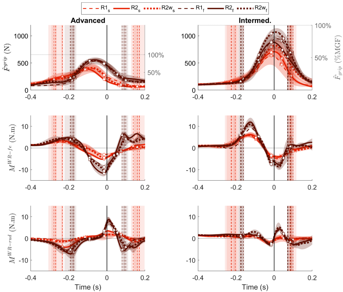
Figure 3. Mean time-patterns (N=5 trials) of estimated grip force ( \hat{F}^{grip} ) and wrist flexion/extension ( M^{WR-fe} ) and radial-ulnar deviation ( M^{WR-rud} ) moments during the forehand drives of both players (Advanced and Intermediate) for the two shot speeds (Slow and Fast) performed with the three rackets (R1, R2, R2w). Shaded areas represent \pm one standard deviation around the mean. Lighter nuances represent the Slow (s) speed shots and darker nuances the Fast (f) ones. The vertical solid black bar represents the impact frame, the dashed vertical bars represent the beginning and end of forward acceleration phase, and the different points correspond to the frames on which musculoskeletal model was run (see corpus). Normalised \hat{F}^{grip} values expressed in percentage of maximal grip force (MGF) are represented on the right axis of upper panels. Wrist moment components are expressed from an internal point of view, such that positive values represent a flexion and ulnar moment exerted by muscles.
