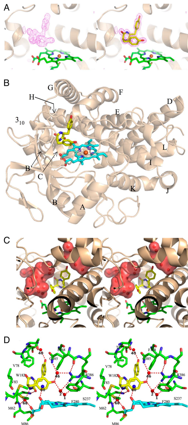
Fig. 4. Crystal structure of cYY-bound CYP121. (A) Fo-Fc electron density map contoured at 4\sigma level (pink) was calculated after 20 cycles of refinement upon removal of the ligand. The overall structure of CYP121 is in cartoon mode colored in wheat, the heme and Cys-345 are represented as sticks and colored in green, with oxygen, nitrogen and sulfur in red, blue and pale yellow, respectively. (Left) Representation of the active site after removal of cYY. (Right) The refined cYY is represented as sticks and colored in yellow (carbon atoms), red (oxygen atoms), and blue (nitrogen atoms). (B) The complex is shown in cartoon representation, with the heme and cYY represented as sticks. The CYP121 backbone is in wheat. The heme is in cyan with the iron in orange, and the cYY is in yellow, with oxygen atoms in red and nitrogen atoms in blue. The helices are labeled according to the previously published CYP121 crystal structure (10). (C) A stereoview of the active site highlighting
