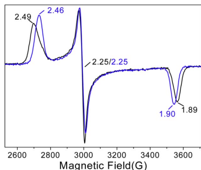
Fig. 2. EPR features of the LS ferric heme of cYY-bound CYP121. 9-GHz EPR spectra of substrate-free CYP121 (black) and CYP121 after addition of a 2-fold excess of cYY (blue) were recorded at 20 K under non-saturating conditions using a microwave power of 0.05 mW and a modulation amplitude of 16 G.
