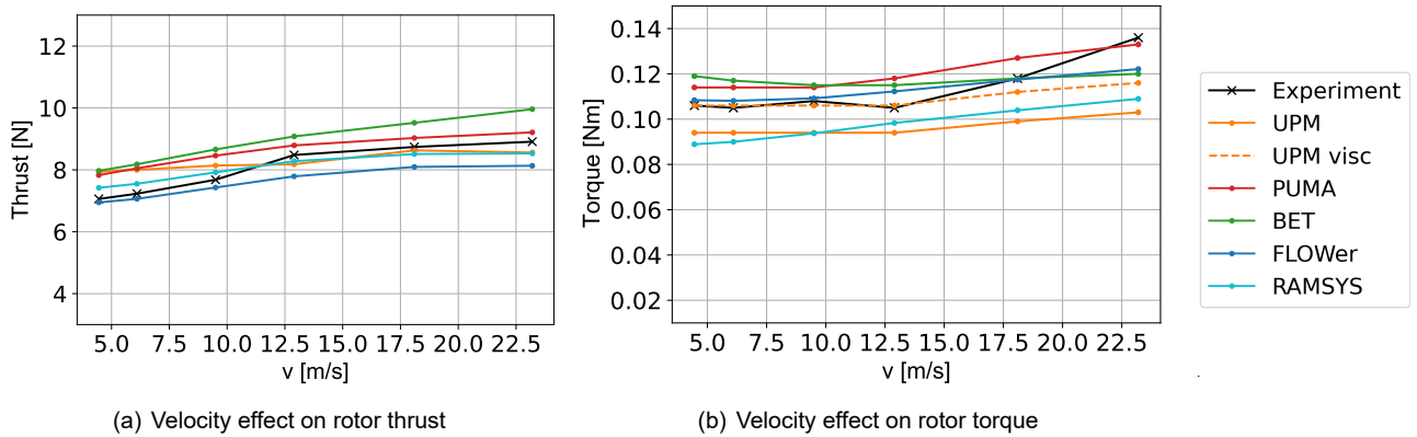
Figure 15: Results for varying rotor velocity with fixed 5900 RPM and tilt angle -10^\circ
