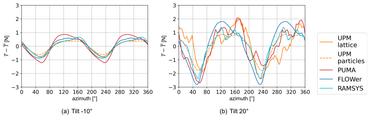
Figure 17: Thrust fluctuations during one rotation for 5400 RPM and flight velocity 12.9 m/s
