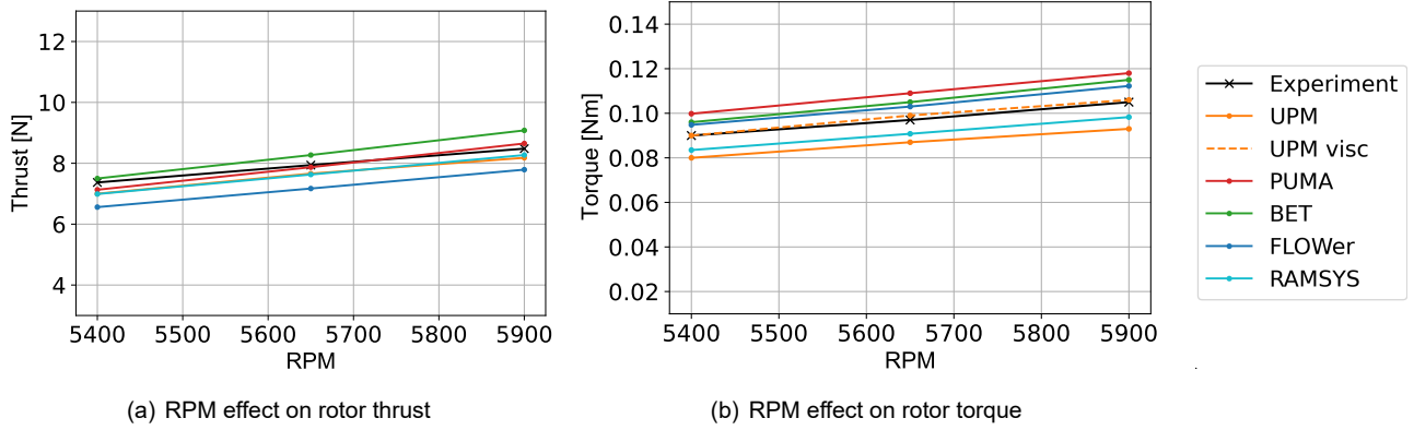
Figure 14: Results for varying rotor RPM with fixed flight velocity of 12.9 m/s and tilt angle -10^\circ
