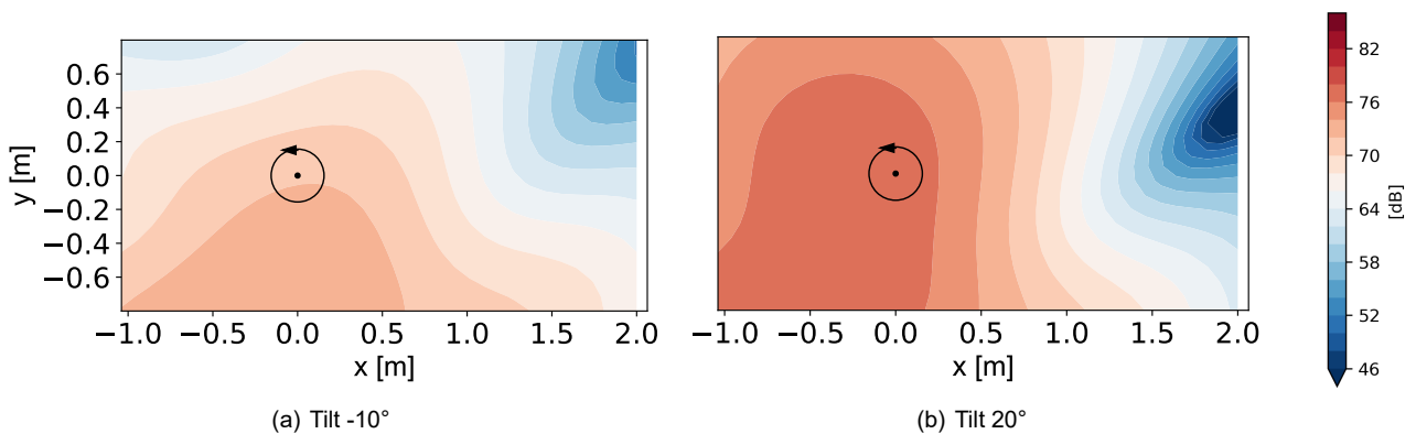
Figure 30: Scattering effects for 5400 RPM and flight velocity 12.9 m/s
