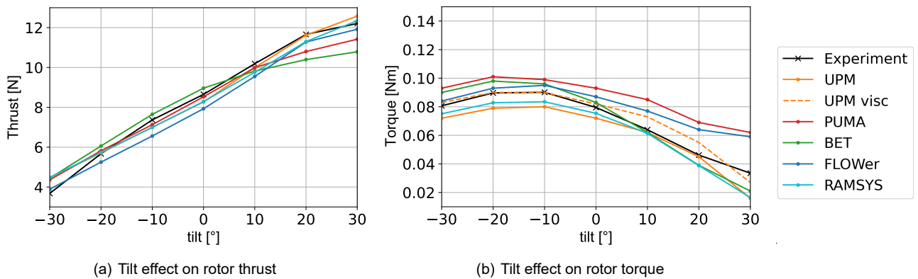
Figure 16: Results for varying rotor tilt angle with fixed 5400 RPM and flight velocity 12.9 m/s
