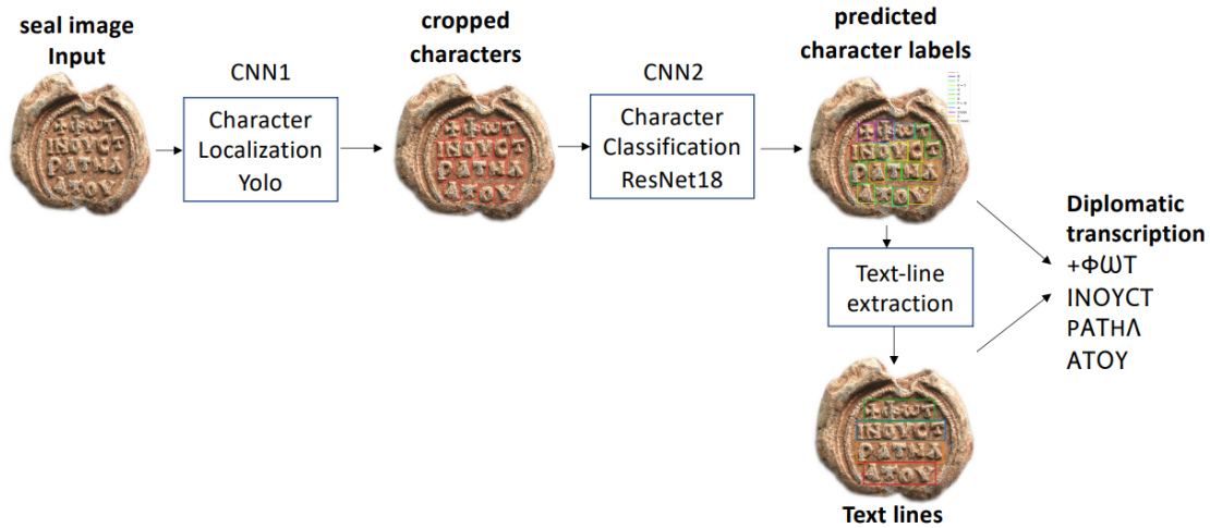
Figure 4: Pipeline of the proposed two-stage character recognition approach. CNN1 is an object detector, while CNN2 is a deep classifier. The output is the plain transcription of the input reverse seal image.
