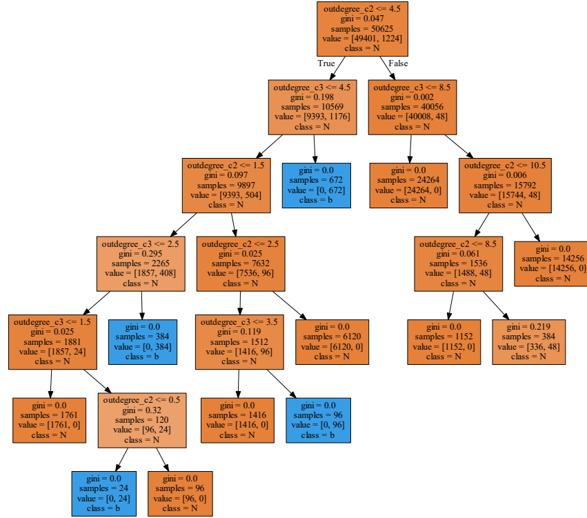
Fig. 7. A decision tree model to predict the existence of a periodic attractor. Blue leaves represent the models classified as having a periodic attractor and orange leaves represent the models classified as not having a periodic attractor. “gini” describes the purity of models in a node regarding the two classes considered here: models having a periodic attractor and models not having a periodic attractor; if all models in a node belong to the same class then \text{gini} = 0 , otherwise \text{gini} > 0 ( \text{gini} = 1 - (\frac{\text{number}_{class1}}{\text{number}_{total}})^2 - (\frac{\text{number}_{class2}}{\text{number}_{total}})^2 ). “sample” represents the number of models in a node. The first value of “value” represents the number of models not having a periodic attractor and the second value of “value” represents the number of models having a periodic attractor.
