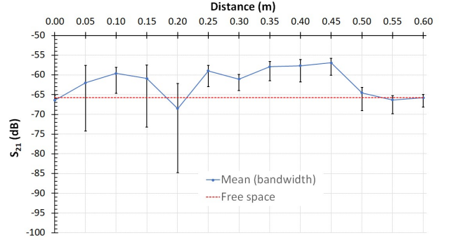
Fig. 6 Effect of the distance between auxiliary box and roof
