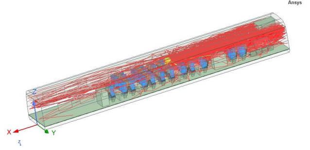
Fig. 10 Ray tracing example in the WLCN simulation
