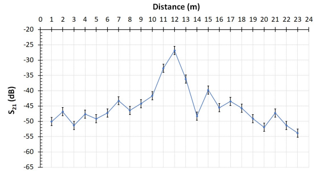
Fig. 11 Sensor position moving along the train car
