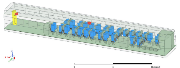
Fig. 2 Train model for WLCN
