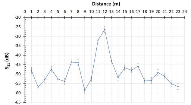
Fig. 12 Camera position moving along the train car
