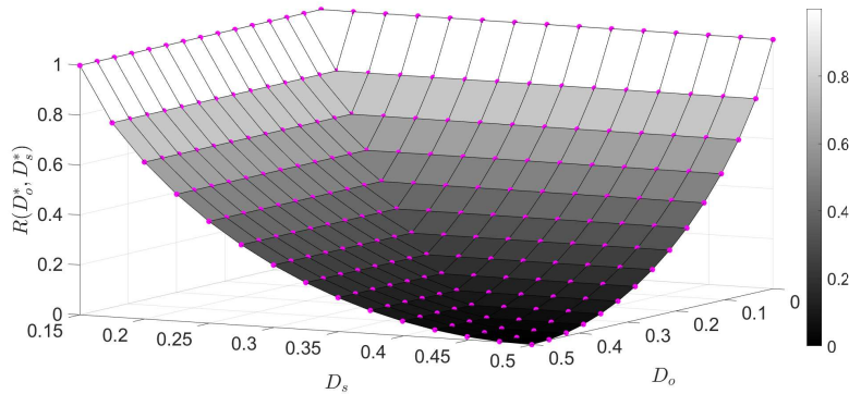
Fig. 2: R(D_o^*, D_s^*) for binary alphabets with an equiprobable semantic source and binary symmetric channel with c = 0.15 .
