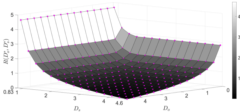
Fig. 3: R(D_o^*, D_s^*) for jointly Gaussian RVs with individual MSE distortion constraints.
