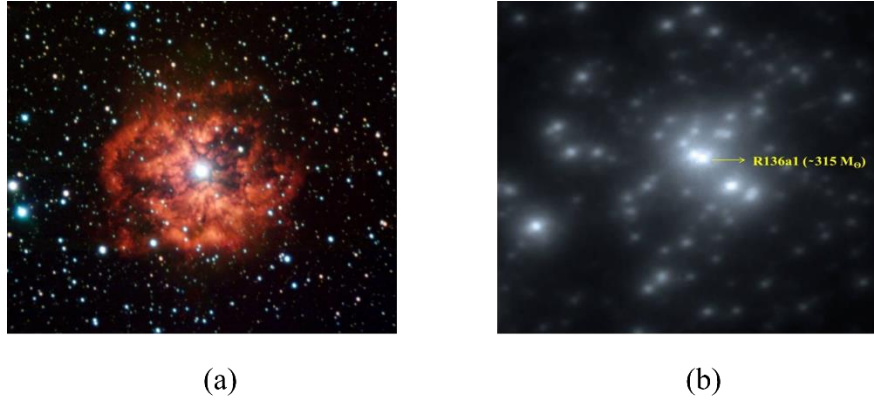
Figure 5. (a) WR 124 in the M1-67 wind-nebula in the Sagittarius constellation, (b) A near-infrared image of the R136 star concentration of the Tarantula Nebula in the Large Magellanic Cloud, obtained at high resolution with the Multi-conjugate Adaptive optics Demonstrator (MAD) at ESO's Very Large Telescope ( Credit. NASA & ESO ).
