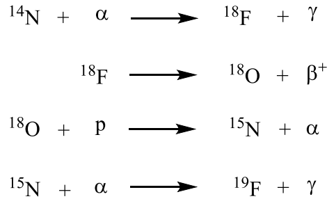
Scheme 3. Nucleosynthetic pathway for ^{19}\text{F} in AGB stars.
