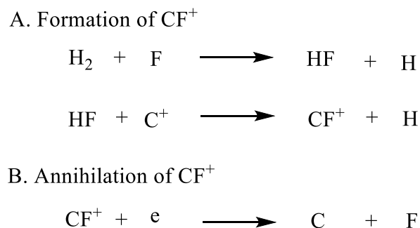
Scheme 4. Formation and annihilation pathways for fluoromethyldynium ion ( \text{CF}^+ ).
