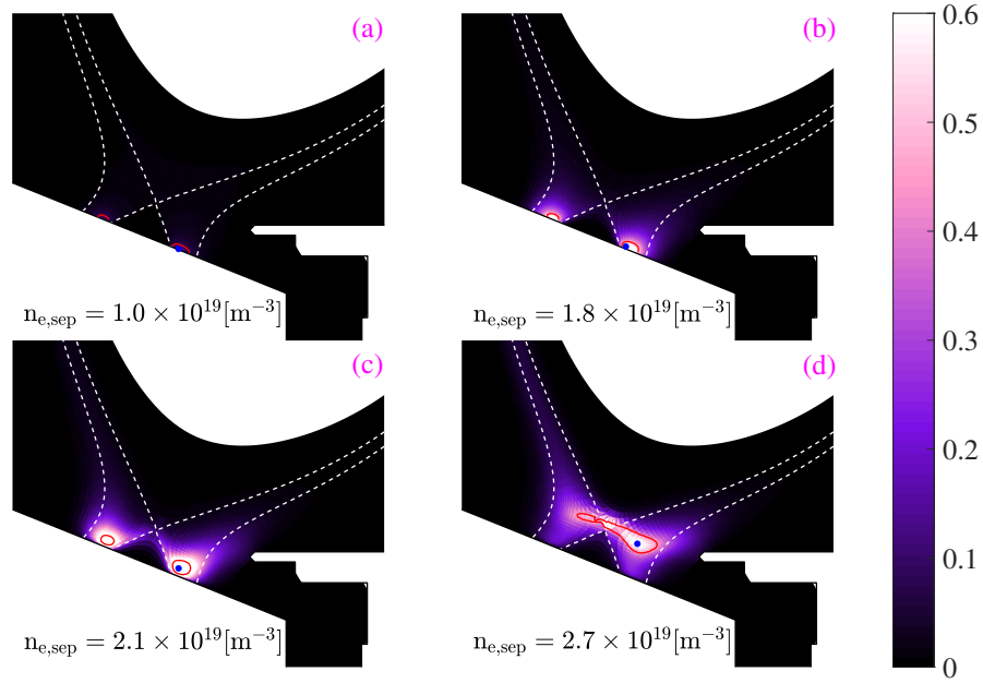
FIGURE 3.37. : Radiation power [ \text{MW}/\text{m}^3 ] in WEST case with closed baffle. With increasing upstream n_{e,\text{sep}} , the main radiation regions surrounded by the radiation fronts (composed of the points that have less than 30% reduced radiation compared to the maximum radiation in the simulation domain, marked by red curve) move up off the divertor target, and two radiation centers on the inner and outer leg merged together near the X-point in the deeply detached regime. The blue dot represents the position where it has the maximum radiation. The white dashed curves represent the separatrix.
