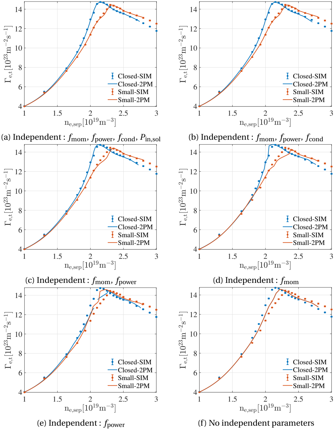
FIGURE 4.19. : Evolution of particle flux at the outer target \Gamma_{e,t} as a function of n_{e,\text{sep}} . Solid curves represent the result from the extended 2PM, scatter points represent the result from SOLEDGE3X-EIRENE simulation (SIM). Here we show only two cases as an example : the case with closed baffle and the case with small leakage under the baffle. Each figure shows the result with different groups of independent input parameters in the extended 2PM. Except for the independent parameters used, other parameters are set to be the common parameters.
