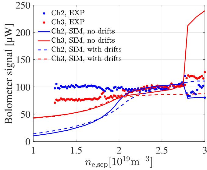
FIGURE 3.22. : Evolution of bolometer signal (Channel 2 and Channel 3) as a function of n_{e,\text{sep}} in WEST discharge #56420, compared with simulation results.
