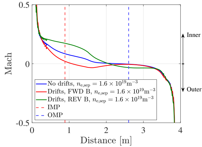
(b) Medium n_{e,sep}
