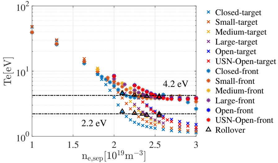
FIGURE 4.12. : The scatter points of the peak electron temperature at the outer target (marked by crosses) and the average electron temperature inside the radiation front (marked by asterisks). The black triangle on each curve marks the point when the rollover of \Gamma_{e,t} happens.
