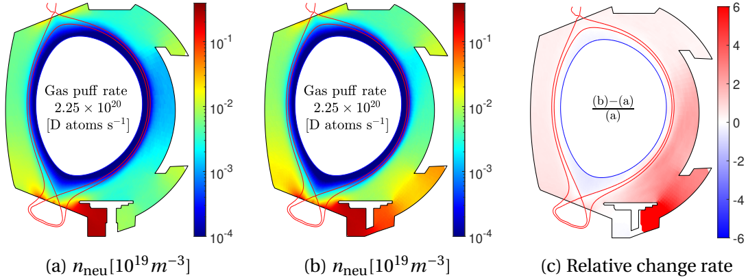
FIGURE 4.6. : (a) The neutral density n_{neu} distribution in the case with closed baffle. (b) The neutral density n_{neu} distribution in the case with small leak. Both (a) and (b) have the same setup parameters include the same gas puff rate = 2.25 \times 10^{20} \text{ atoms s}^{-1} . (c) The contour of relative change rate in neutral density n_{neu} shows that the leakage under baffle results in the increase of neutral density by a factor of 2.5–6 in the LFS and of 1.5 in the high field side of the main chamber.
