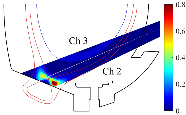
FIGURE 3.20. : The contour of radiation [MW/m 3 ], with channel 2 and channel 3 marked.
