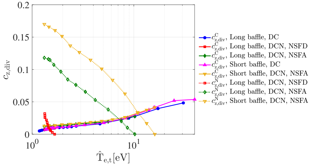
FIGURE 4.32. : Evolution of carbon and nitrogen concentration ( c_{z,\text{div}}^C and c_{z,\text{div}}^N , respectively) as a function of peak electron temperature \hat{T}_{e,t} at the outer target.
