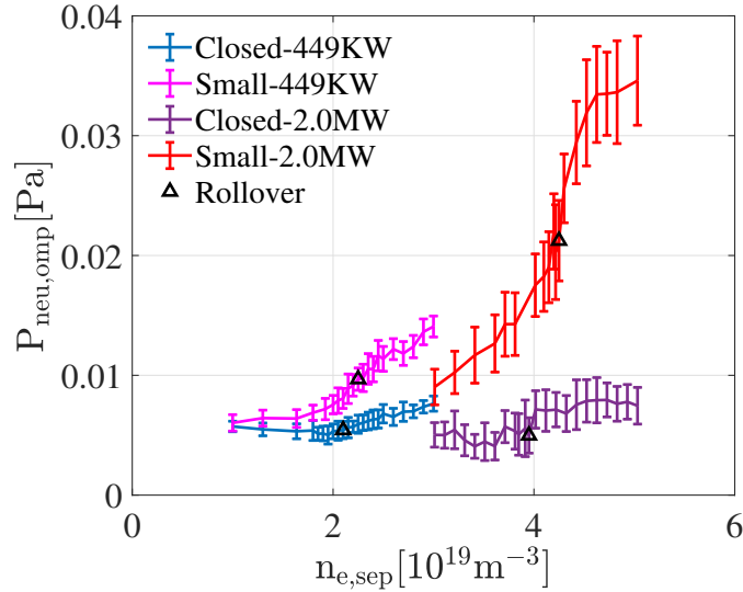
FIGURE 4.50. : Evolution of the average neutral pressure the near-wall OMP. The black triangle on each curve marks the point when the rollover of \Gamma_e happens.
