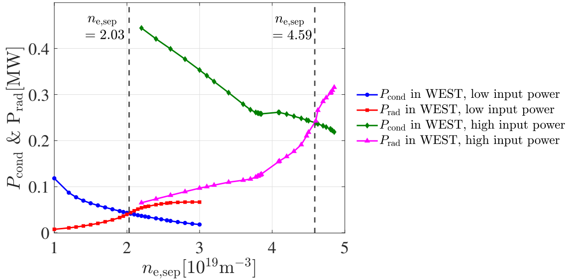
FIGURE 5.2. : Evolution of radiation and conductive power at divertor outer leg in WEST as a function of n_{\text{e,sep}} .
