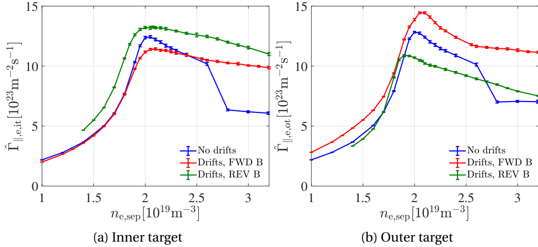
FIGURE 23. : Evolution of peak parallel particle flux at inner (outer) target as a function of n_{\text{e, sep}} in no drifts, forward \mathbf{B}_\phi , and reversed \mathbf{B}_\phi cases.
