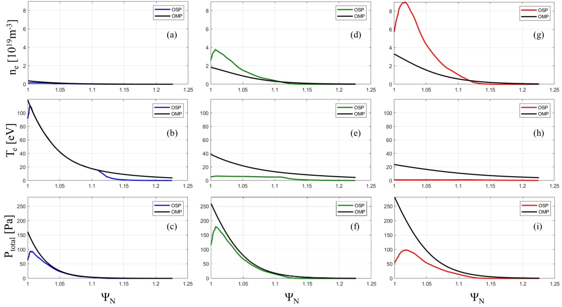
FIGURE 2.8. : The three columns from left to right correspond to the n_{e,\text{sep}} from low to high value : n_{e,\text{sep}} = 3.60 \times 10^{18} \text{ m}^{-3} , n_{e,\text{sep}} = 1.85 \times 10^{19} \text{ m}^{-3} , and n_{e,\text{sep}} = 3.30 \times 10^{19} \text{ m}^{-3} . The three rows from top to bottom show the comparison of the electron density, temperature, and total pressure profiles at the OMP and the outer divertor target. The curves in colors (blue, green, and red) represent the profiles at the target, while the black curves represent the profiles at the OMP.
