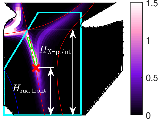
FIGURE 3.39. : 2D map of P_{\text{rad}} [MW/m 3 ], the same case as (f) in Figure 3.38. For the outer divertor, the radiation front (marked by red cross) is defined as the lowermost point of a region (enclosed by green curve) inside which the P_{\text{rad}} of each point is higher than 70% of maximum radiation in the analyzed spatial domain (marked by cyan polygon). The height of the radiation front H_{\text{rad,front}} and the height of X-point H_{\text{X-point}} are defined as the vertical distance between the outer target and the radiation front or X-point, respectively.
