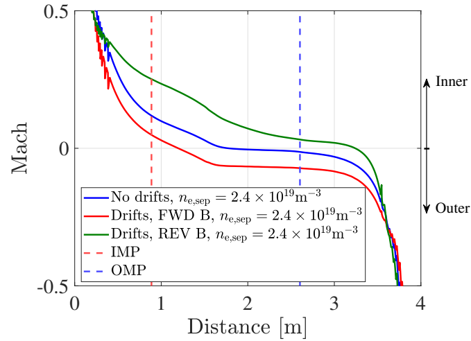
(c) High n_{e,sep}
