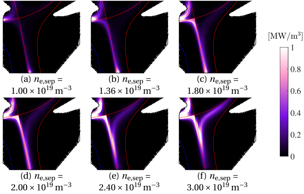
FIGURE 3.38. : 2D maps of P_{\text{rad}} , from (a) to (f) with increasing n_{\text{e,sep}} . In order to highlight the radiation front region, the upper limit of color bar is set as 1 \text{MW}/\text{m}^3 , even if the peak value of radiation can be 10 \text{MW}/\text{m}^3 , occur at the inner target, in some cases.
