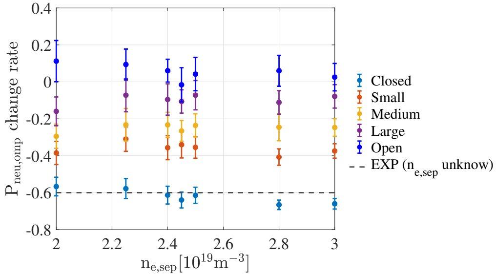
FIGURE 4.22. : The change rate of the neutral pressure at the near wall OMP : (P_{neu,omp}^{LSN} - P_{neu,omp}^{USN})/P_{neu,omp}^{USN} , as a function of upstream n_{e,sep} . The dashed line represent the P_{neu,omp} change rate = -0.6 , comparing between discharges #56726 and #56769.
