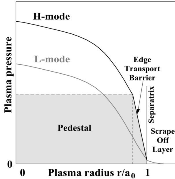
FIGURE 1.5. : Typical pressure profiles observed in L- and H-mode phases. Figure from reference [18].
