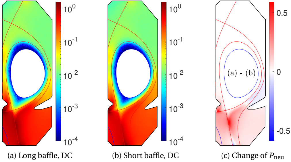
FIGURE 4.28. : 2D maps of P_{\text{neu}} [Pa] are shown in (a) and (b), which have the same upstream separatrix density ( n_{\text{e,sep}} = 3 \times 10^{19} \text{ m}^{-3} ) but different baffle lengths. Plot (c) shows the change in neutral pressure between (a) and (b) when the baffle length is increased while keeping n_{\text{e,sep}} constant.
