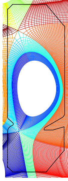
FIGURE 3.29. : SOLEDGE3X mesh grid based on magnetic configuration of #70690 at t = 1 s in TCV.
