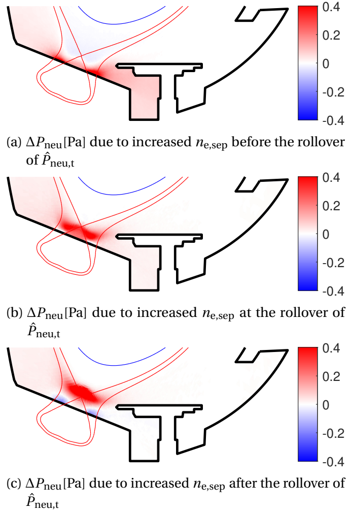
FIGURE 4.9. : The 2D maps (a)–(c) represent the change of neutral pressure \Delta P_{\text{neu}} in the lower divertor when upstream density increases by a little \Delta n_{\text{e,sep}} = 2.0 \times 10^{18} \text{ m}^{-3} in the case with baffle closed : (a) represents the result before the rollover of peak neutral pressure at the divertor outer target \hat{P}_{\text{neu,t}} with an increase of n_{\text{e,sep}} by \Delta n_{\text{e,sep}} from 1.80 \times 10^{19} \text{ m}^{-3} . (b) represents the result at the rollover of \hat{P}_{\text{neu,t}} with an increase of n_{\text{e,sep}} by \Delta n_{\text{e,sep}} from 2.25 \times 10^{19} \text{ m}^{-3} . (c) represents the result after the rollover of \hat{P}_{\text{neu,t}} an increase of n_{\text{e,sep}} by \Delta n_{\text{e,sep}} from 2.80 \times 10^{19} \text{ m}^{-3} .
