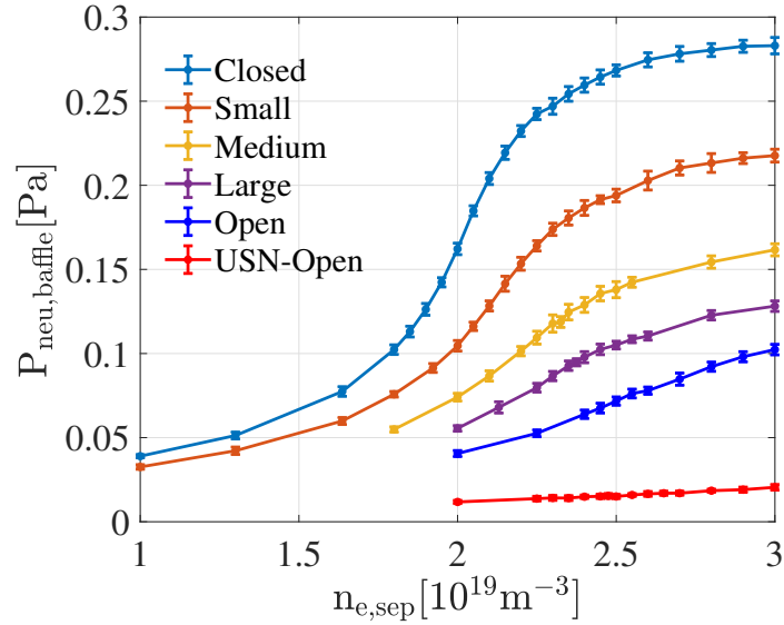
FIGURE 4.20. : Evolution of neutral pressure under baffle as a function of upstream n_{e,sep} .
