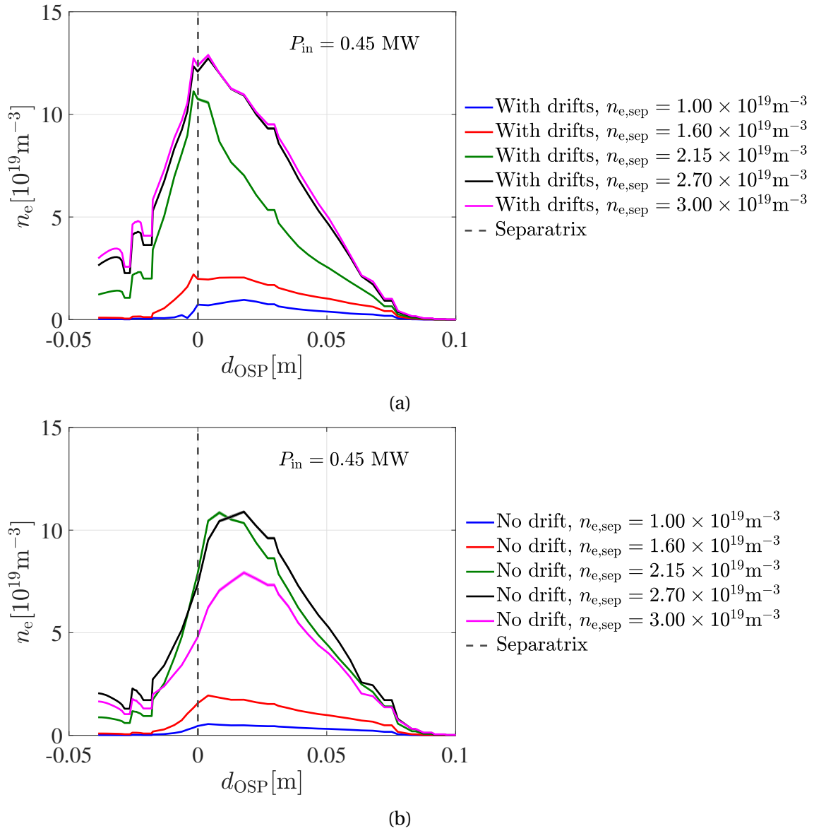
FIGURE 4.42. : (a) Evolution of density profile at the outer target with increasing n_{e,\text{sep}} in the low input power case with drifts. (b) Evolution of density profile at the outer target with increasing n_{e,\text{sep}} in the low input power case with no drifts. d_{\text{OSP}} is the radial distance from the outer strike point, negative values are in the PFR, positive values are in the SOL. The dashed line represents the position of separatrix.
