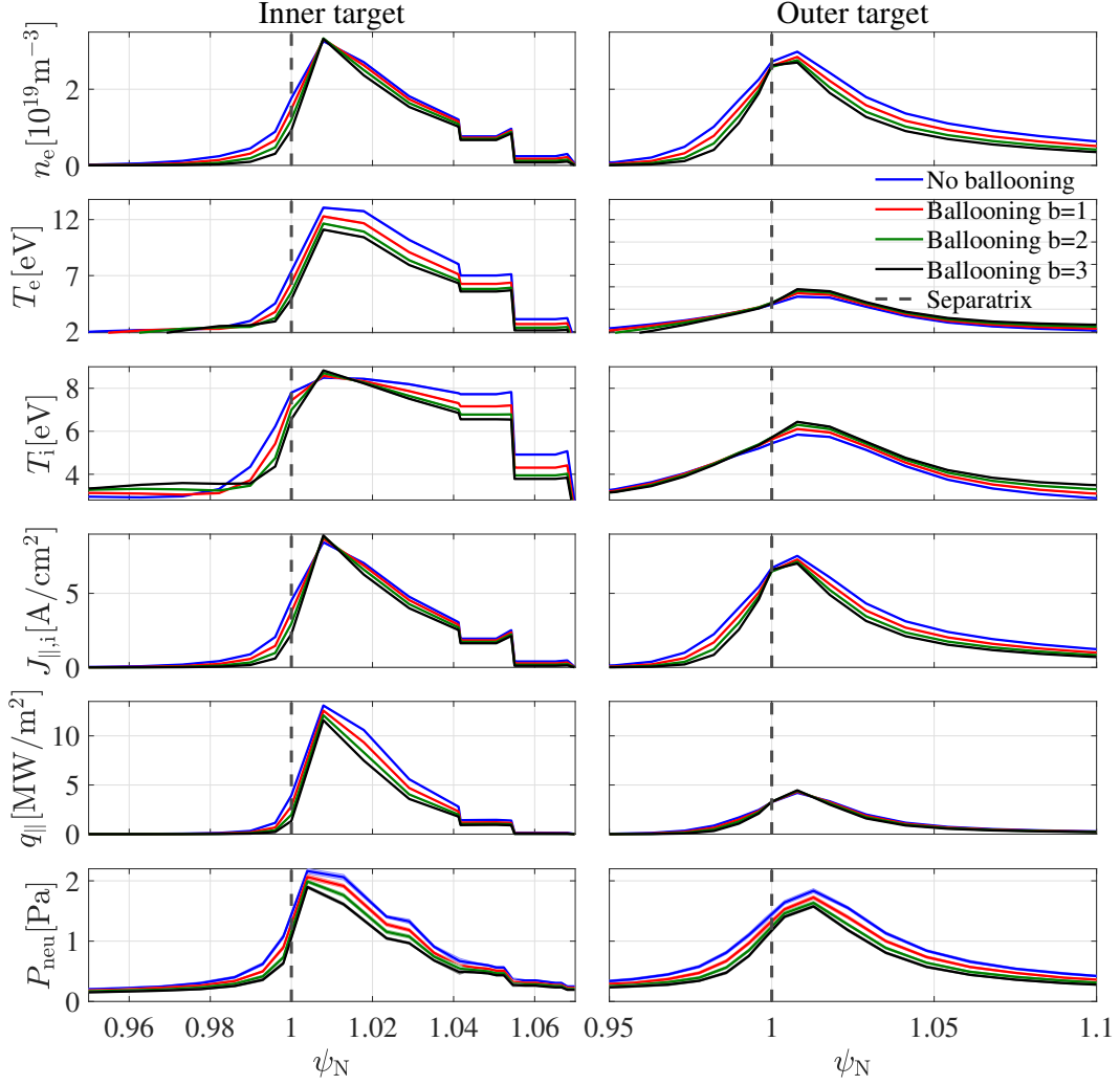
FIGURE 14. : The impact of ballooning at the target profiles in TCV case.
