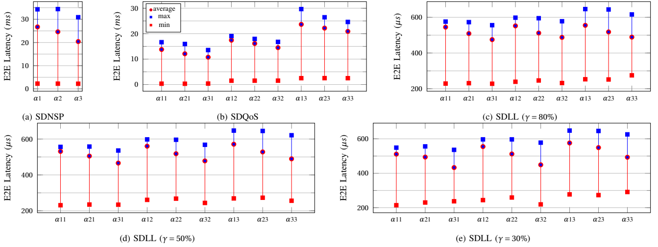
Figure 4: Scenario 1 E2E latency results experienced by (HP, MP, LP) packets ( \alpha_{ij} ) and handled by SDNSP and SDQoS static solutions, and SDLL framework with different threshold ( \gamma ) and number of packets ( \alpha_{ij} ).
