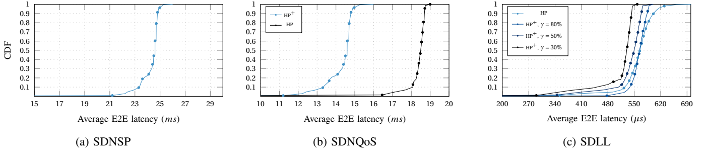
Figure 5: Scenario 2 E2E latency results experienced by HP and HP + packets when using SDNSP, SDQoS and SDLL with \gamma = (80\%, 50\%, 30\%) for HP packets.
