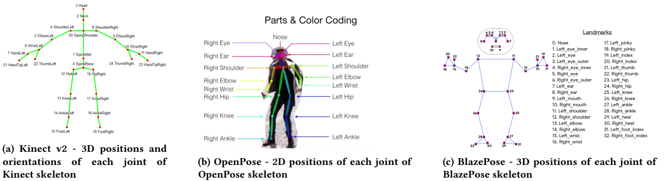
Figure 5: Skeletons
