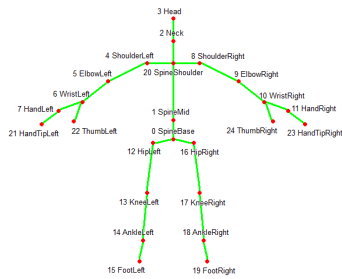
Figure 2: Kinect skeleton
