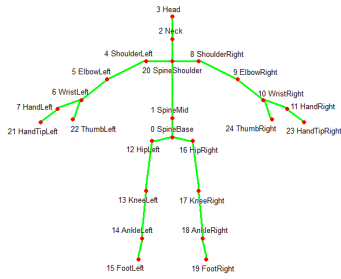
Figure 2: Kinect skeleton
