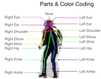
Figure 3: OpenPose skeleton
