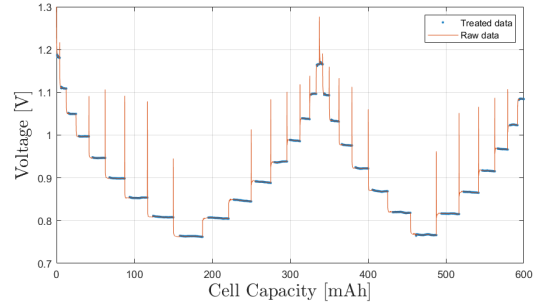
Fig. 7. Output voltage fragments after data treatment.
