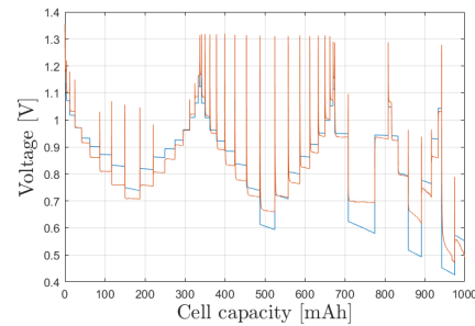
Fig. 11. Comparison of the model output to the validation data profile.
