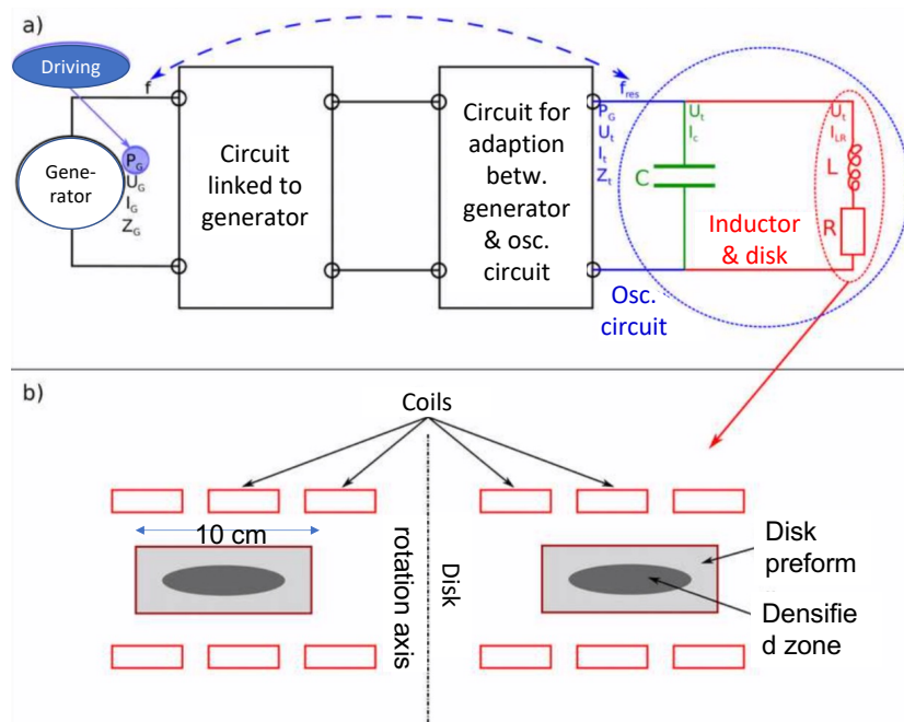
Figure 8: Description of the RF heating system. a) Equivalent electrical circuit; b) the inductor-preform system, equivalent to an RL device.
