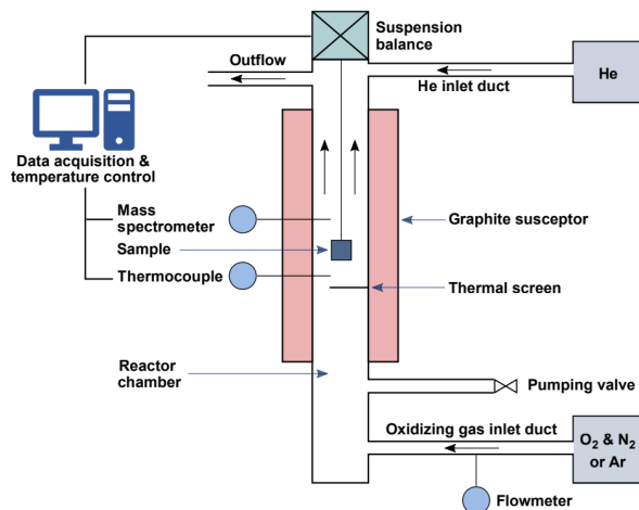
Figure 2: Diagram of the TGA equipment. *color should be used for that figure.*
