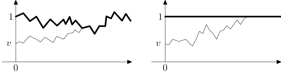
FIGURE 1. On the left: \text{BESQ}^{\delta, \delta'} flow. The process x \rightarrow f(x) is traced in bold. A flow line x \rightarrow S_{0,x}(v) is also represented. On the right: \text{Jacobi}(\delta, \delta') flow after a space-time transformation. The process x \rightarrow f(x) is mapped to the constant function 1, and the image of the flow line at v is a flow line of the Jacobi flow.
