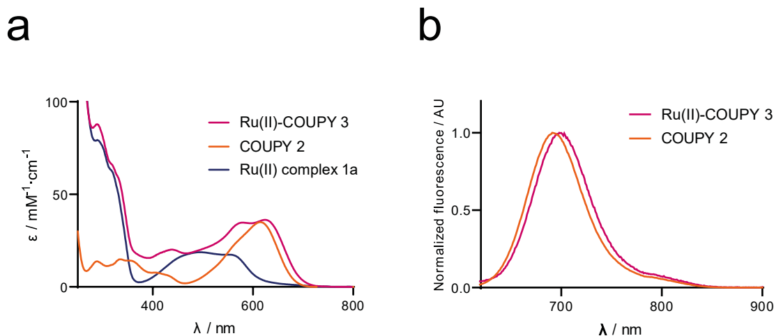
Figure 2. Comparison of the molar absorptivity of the Ru(II)-COUPY conjugate 3 with that of the unconjugated parent compounds ( 1a and 2 ) in ACN ( a ) and emission spectra of 2 and 3 after excitation at 600 nm in ACN ( b ).
