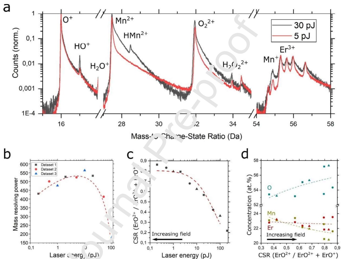
Figure 2: Influence of Ar \Gamma parameter on key analysis metrics. (a) Mass spectrum of \text{ErMnO}_3 for two different laser energies, 5pJ and 30pJ (see Figure S4 for a full spectrum). Thermal tails are reduced at 5pJ compared to 30pJ. (b) MRP as a function of the laser energy from three different APT specimens (distinguished by colors). All data is acquired under the same parameters aside from the laser energy (i.e. base temperature: 50K, detection rate: 0.5%, pulse frequency: 250 kHz). (c) CSR evolution of the ErO ionic species ( \text{ErO}^{2+} and \text{ErO}^+ ) as a function of the laser energy. (d) Composition of the full data volume as a function of CSR. Increasing CSR corresponds to reducing the laser energy. In both (c) and (d) the arrow indicates the direction of which the electric field strength increases, and the plotted lines are guides to the eye. All three plots (b-d) show that analysis conditions are improved towards lower laser energies (<10pJ).
