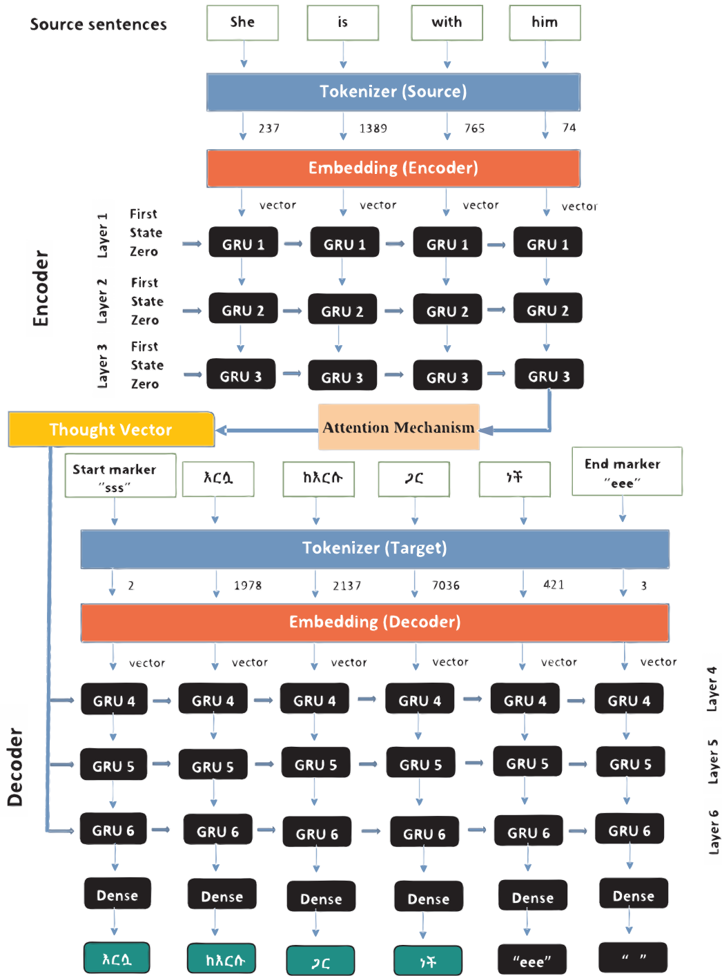
Figure 2: GRU model architecture.
