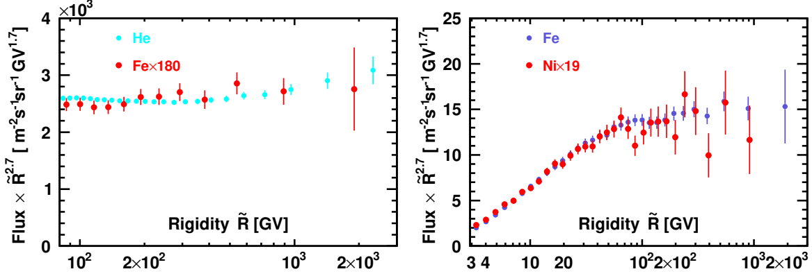
Figure 5: Left panel: The rigidity dependence of the Fe flux compared to the rigidity dependence of the He flux above 80.5 GV. Right panel: The rigidity dependence of the Ni flux compared to the rigidity dependence of the Fe flux above 3 GV.
