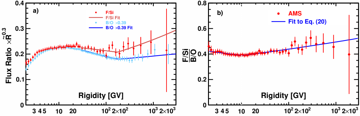
Figure 11: Left panel: The AMS F/Si flux ratio and AMS B/O flux ratio as functions of rigidity with total errors. For display purposes only, the F/Si and B/O flux ratios are multiplied by \tilde{R}^{0.3} and the B/O flux ratio rescaled as indicated. The solid red and blue curves show the F/Si and B/O fit results with Eq. (4), respectively. Right panel: The AMS \frac{F/Si}{B/O} ratio as a function of rigidity with total errors. The solid blue curve shows the fit results of Eq. (4). As seen, the rigidity dependence of F/Si and B/O flux ratios are distinctly different. Above 10 GV the \frac{F/Si}{B/O} ratio can be described by a single power law \propto R^\delta with \delta = 0.0525 \pm 0.0065 ( a > 7\sigma difference from zero).
