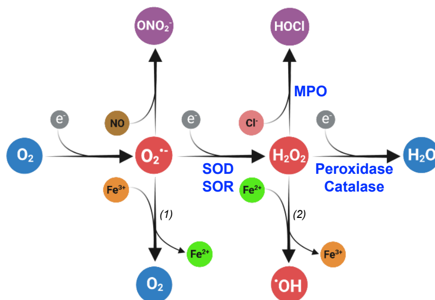
Figure 1. Superoxide ( O_2^{\bullet-} ), hydrogen peroxide ( H_2O_2 ), and hydroxyl radical ( \bullet OH ) are reactive oxygen species (ROS) produced by the subsequent reduction in dioxygen ( O_2 ). In living organisms, the dismutation or reduction in superoxide, catalyzed by superoxide dismutase (SOD) and reductase (SOR), respectively, gives rise to hydrogen peroxide. Peroxidases and catalase catalyze the hydrogen peroxide reduction or dismutation, respectively, into water. Superoxide can react with nitric oxide (NO) to form peroxynitrite ( ONO_2^- ), and hydrogen peroxide can be transformed into hypochlorous acid (HOCl) in a reaction catalyzed by myeloperoxidases (MPO). The reactions (1) and (2) constitute the Haber–Weiss reaction that produces dioxygen and hydroxyl radical from superoxide and hydrogen peroxide, respectively. The reaction (2) is the Fenton reaction. Created with BioRender (BioRender.com).
