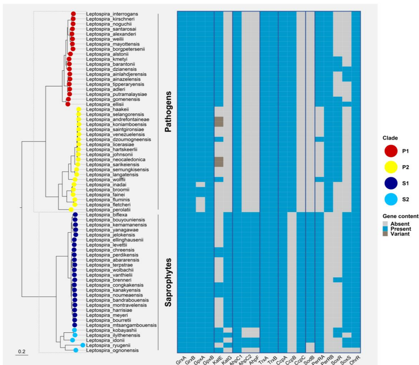
Figure 4. Phylogenetic distribution of ROS defenses and ROS-responsive regulators in all Leptospira spp. Ortholog sequences for each protein were searched with both BLAST v2.13.0 and HMMer v3.3.1 against a database of reference proteomes for the 68 Leptospira spp. with an e-value cut-off of 0.01 [72,73]. Alignments were performed with MAFFT v7.467 using the L-INS-i algorithm and tree inference was computed with FastTree v2.1.1 [74]. Direct homologs of the target protein were manually curated and selected from this phylogeny. These homologs were finally mapped to a core-genome tree of Leptospirales constructed based on a concatenated alignment of 1576 marker genes (identified with standalone OMA v2.5.0) and inferred with IQ-TREE v2.0.6 under the best-fit model of evolution (LG+F+R8) [75,76]. Leptonema illini and Turneriella parva were used as a root for the final Leptospira spp. phylogeny. The final figure was generated using the ggtree package for R [77]. Grx: glutaredoxins; GPx: glutathione peroxidase; KatE: catalase HPII; katG: catalase HPI; AhpC: Alkyl hydroperoxidase or Alkyl hydroperoxide reductase; AhpF: AhpC reductase; Trx: thioredoxin; Ccp: cytochrome C peroxidase; Sod: superoxide dismutase; PerR: peroxide stress regulator; SoxR: transcriptional activator and sensor of superoxide; SoxS: transcriptional activator of the SoxR regulon; OhrR: organic hydroperoxide resistance regulator.
