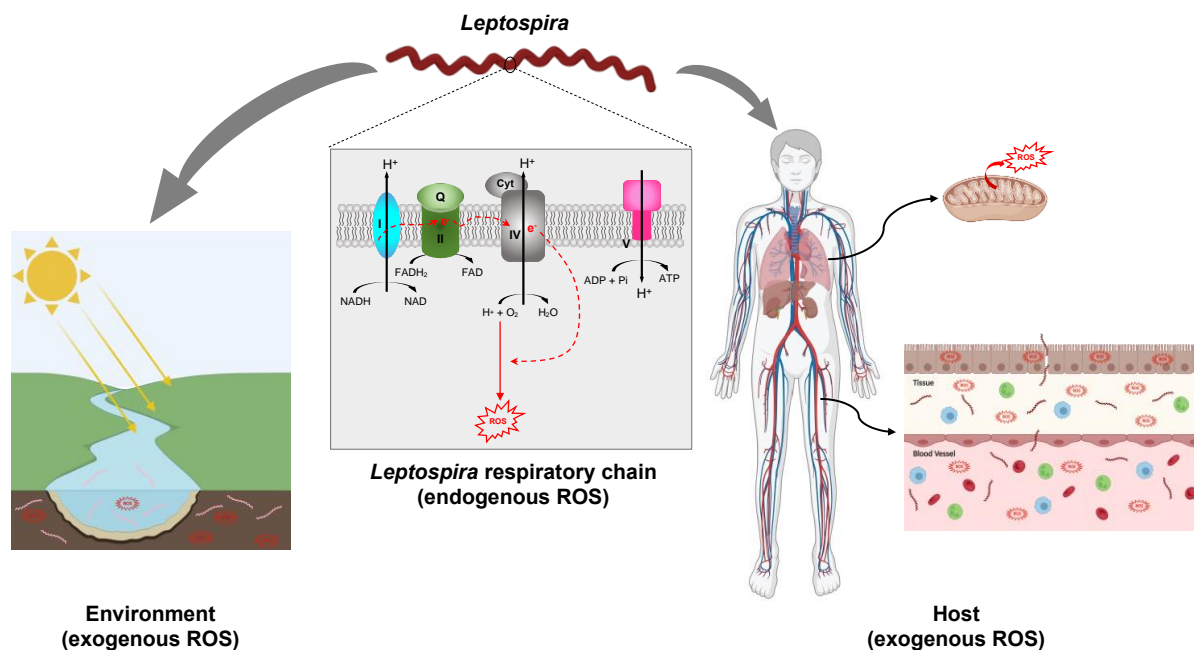
Figure 2. Exposition of Leptospira to ROS. Leptospira spp. are potentially exposed to ROS produced endogenously as a result of electron leakage from the respiratory chain. The putative complexes forming the respiratory chain in pathogenic Leptospira , complex I (encoded by LIMLP_00745-00750, LIMLP_03705-03760 in L. interrogans serovar Manilae), complex II (encoded by LIMLP_09980-09990 in L. interrogans serovar Manilae), complex IV (encoded by LIMLP_01080-01085, LIMLP_01375, LIMLP_01100-01110 in L. interrogans serovar Manilae), and complex V (encoded by LIMLP_06045-06080 in L. interrogans serovar Manilae) are represented. Leptospira spp. also face ROS produced in the environment (waters and soils). In addition, pathogenic species are exposed to ROS produced by the host phagocytic cells or tissues. The host mitochondria are one of the main ROS producers. Created with BioRender ( BioRender.com ).
