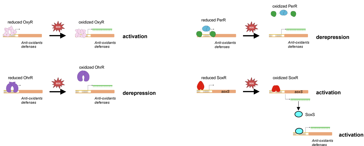
Figure 6. Oxidation-based regulation of DNA binding by oxidative-stress transcriptional regulators. The reduced and oxidized forms of different transcriptional regulators and ROS sensors are schematized in this cartoon. Oxidation of the regulators leads to conformational switch resulting either in a better DNA binding and activation of transcription (as for OxyR, SoxR, and SoxS) or in DNA dissociation and repression alleviation (as for PerR and OhrR).
