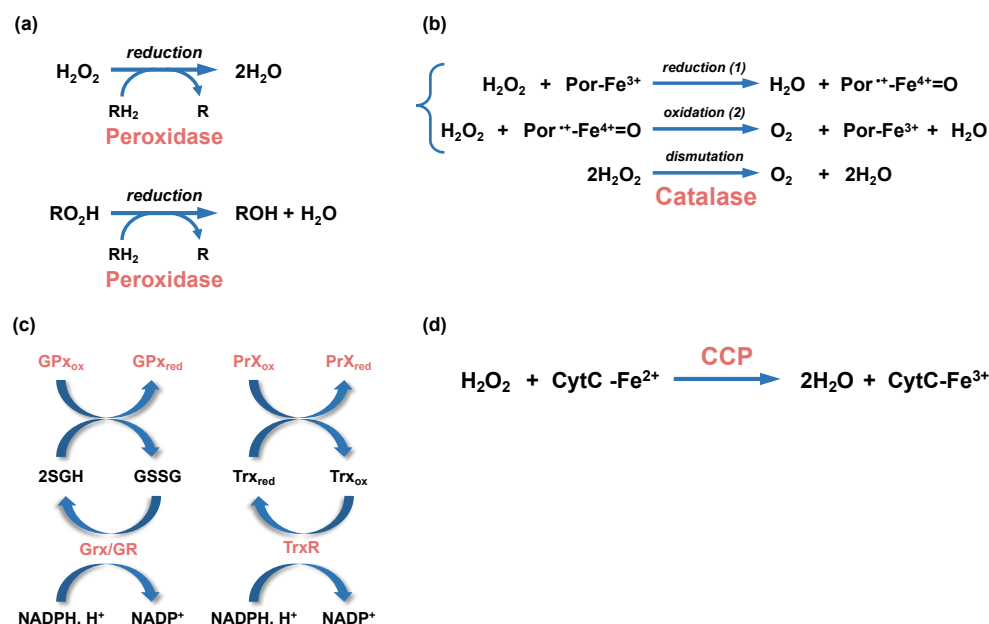
Figure 3. Enzymatic reactions leading to peroxide detoxification. (a) Hydrogen peroxide ( \text{H}_2\text{O}_2 ) and alkyl peroxides ( \text{RO}_2\text{H} ) are reduced by peroxidases (peroxidase or glutathione peroxidases), with the participation of an organic electron donor ( \text{RH}_2 ). (b) The dismutation of \text{H}_2\text{O}_2 into water and dioxygen ( \text{O}_2 ) by heme-using catalases is a two-step reaction. In a first step (1), one molecule of \text{H}_2\text{O}_2 is reduced into water in a reaction where the heme ferric porphyrin ( \text{Por-Fe}^{3+} ) acts as an electron donor and is oxidized into an oxoferryl porphyrin cation radical ( \text{Por}^{\bullet+}\text{-Fe}^{4+=\text{O}} ). In a second step (2), a second molecule of \text{H}_2\text{O}_2 is oxidized into \text{O}_2 , allowing the regeneration of the ferric porphyrin. (c) Glutathione peroxidases (GPx) and glutaredoxin (Grx), which are oxidized during peroxide reduction or glutathionylation, use glutathione (GSH) as cofactors to regenerate their reduced forms, whereas the oxidized peroxidase (PrX ox ) is reduced by thioredoxin (Trx). The glutathione disulfide (GSSG) and oxidized thioredoxin (Trx ox ) produced during these reactions are reduced by the glutathione reductase (GR) and thioredoxin reductase (TrxR), respectively. The NADPH/NADP + is the redox couple involved in these reactions. (d) A simplified \text{H}_2\text{O}_2 reduction reaction by cytochrome C peroxidase (CCP) is represented. The CCP-bound heme is first reduced by the cytochrome C ( \text{CytC-Fe}^{2+} ). The activated CCP reduces \text{H}_2\text{O}_2 into 2 molecules of \text{H}_2\text{O} using the electron of its reduced heme.
