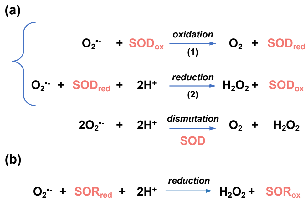
Figure 5. Enzymatic reactions leading to superoxide detoxification. (a) Superoxide dismutase (SOD)-catalyzed dismutation of O_2^{\bullet -} . O_2^{\bullet -} is oxidized into O_2 (reaction 1) and reduced into H_2O_2 (reaction 2). In these reactions, SOD is interconverted between an oxidized ( SOD_{ox} ) and reduced ( SOD_{red} ) forms. (b) Superoxide reductase (SOR)-catalyzed reduction in O_2^{\bullet -} . During the reduction of O_2^{\bullet -} into H_2O_2 , reduced SOR ( SOR_{red} ) is converted into an oxidized form ( SOR_{ox} ).
