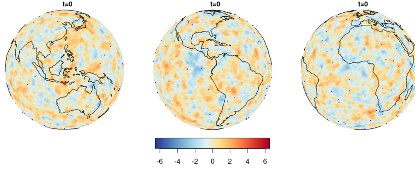
(A) Simulation from which the data are sampled.
