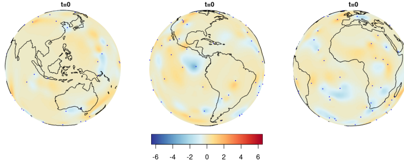
(B) Kriging predictor.
