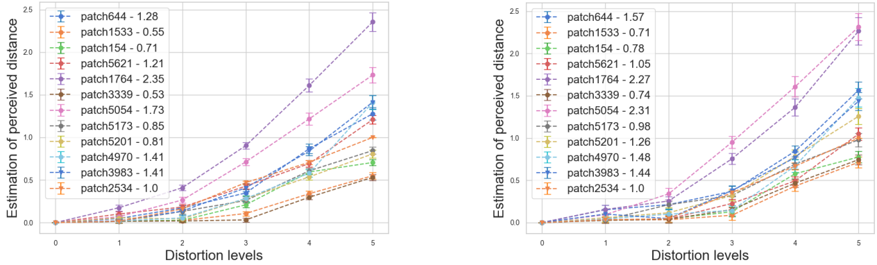
Fig. 2: MLE solving on the two datasets: (left) "in-lab" dataset and (right) "crowdsourced" dataset. Confidence Intervals (CIs) are obtained via bootstrapping [26] over 100 runs. The X-axis is the distortion levels applied on each reference tube, and the Y-axis is the estimated perceived distances by participants between the reference and the distorted tubes.
