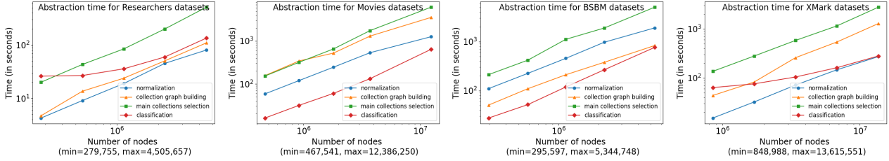
Figure 8: Abstraction computation times on synthetic JSON, PG, RDF and XML datasets, using ( w_{d_{wPR}} , \text{bound}_{fl-ac} ).
