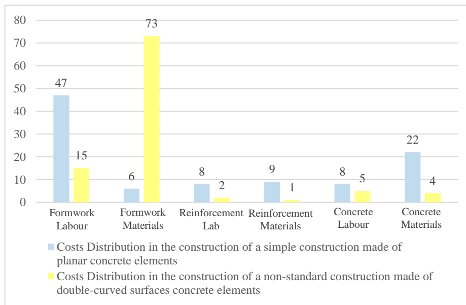
Fig. 1. Costs distribution in the construction of a simple and a complex concrete structure [2], [3].
