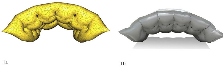
Fig. 4. Simulation of inflated sheets (1a) and fabricated prototype (1b) with the same 2D pattern.
