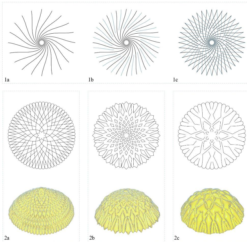
Fig. 9. From an array (1), 3 patterns are drawn (2a, 2b, 2c).
