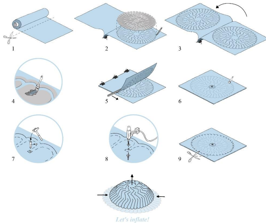
Fig. 11. Protocol of an inflatable fabrication, from step 1 to step 9.
