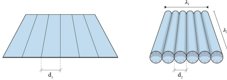
Fig. 5. Two layers sealed according to parallel lines and inflated.
