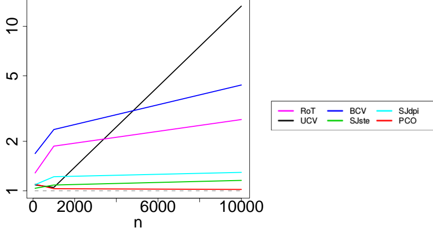
Figure 4: Graph of the mean over all densities f of the ratio of r_{\text{meth}/\min}(f) := \frac{\overline{ISE}_{\text{meth}}^{1/2}(f)}{\min_{\text{meth}} \overline{ISE}_{\text{meth}}^{1/2}(f)} for \text{meth} \in \{\text{RoT}, \text{UCV}, \text{BCV}, \text{SJste}, \text{SJdpi}, \text{PCO}\} with the Gaussian kernel versus the sample size.
