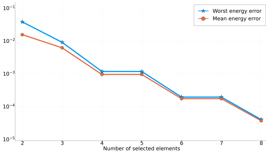
FIG. 5.10. Extrapolation example: decay of the energy error over a set of 21 equally distributed elements for r \in [3.05, \dots, 4] .
