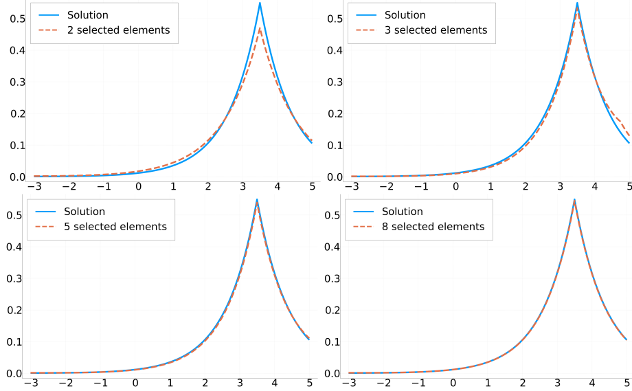
FIG. 5.9. Extrapolation: example of energy projections for r = 3.5 .
