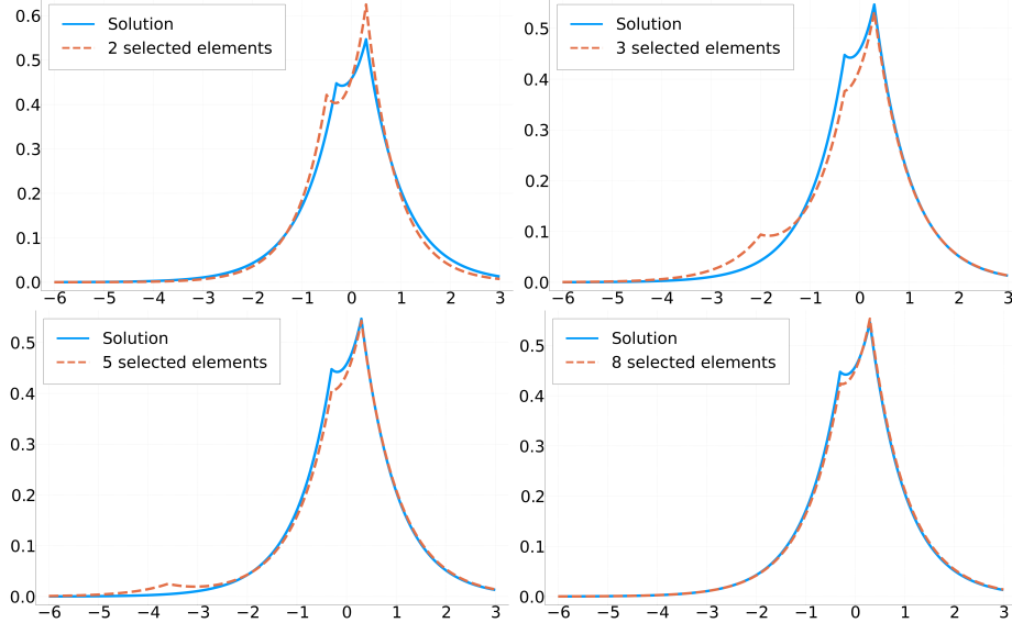
FIG. 5.7. Extrapolation: example of energy projections for r = 0.3 .
