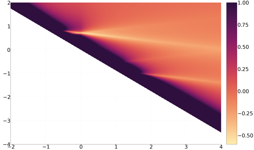
FIG. 5.5. Heatmap of an energy functional (for r = 2.15 ) at barycenters between first two selected elements.
