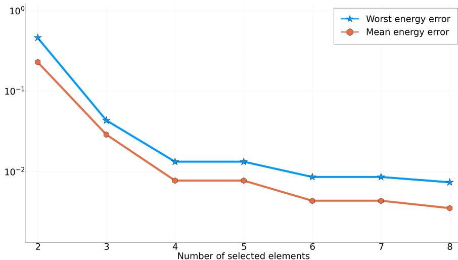
FIG. 5.8. Extrapolation: decay of the energy error over a set of 17 equally distributed elements for r = 0, \dots, 0.48 .
