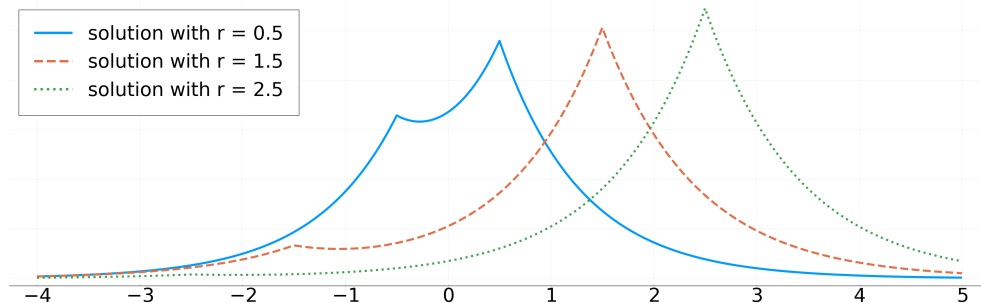
FIG. 5.1. Three example solutions in \mathcal{M}_{tr} .
