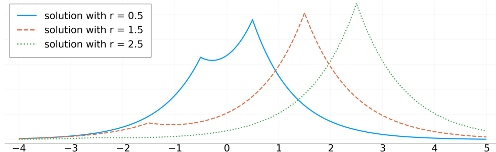
FIG. 5.1. Three example solutions in \mathcal{M}_{tr} .
