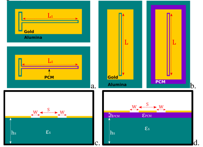
Fig. 1. (a) Design of mmW stub resonators without a PCM (up) and integrating a PCM pattern (down). (b) Example of a CPW line fabricated on an alumina substrate (left) and on a PCM/ alumina layer (right). (c) Cross-section cut of a CPW on an alumina substrate. (d). Cross-section cut of a CPW on a PCM/Alumina substrate.
