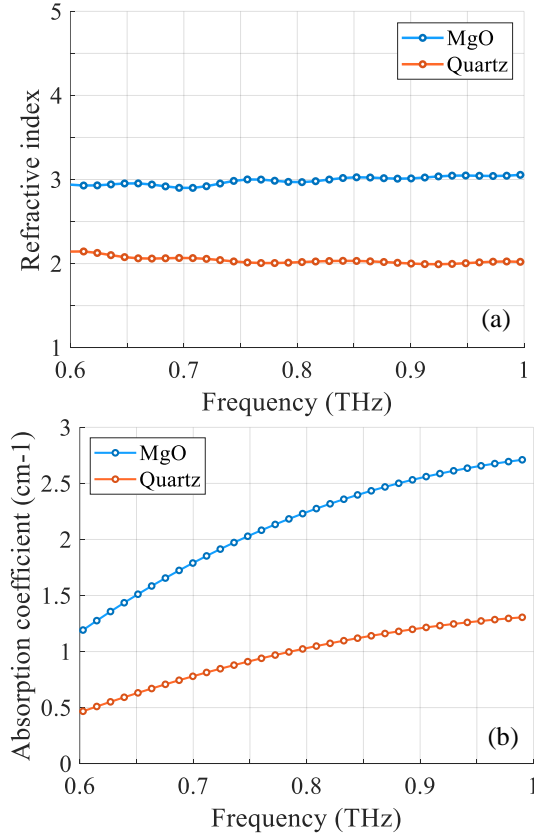
Fig. 9. (a) Frequency dependent refractive index computed from reconstructed data using equation (6) at two different coordinates: MgO at x=6\text{mm} and z=5\text{mm} (blue curve) and quartz at x=-3\text{mm} and z=-3\text{mm} (orange curve). (b) Frequency dependent absorption coefficient computed from reconstructed data using equation (9) at two different coordinates: MgO at x=6\text{mm} and z=5\text{mm} (blue curve) and quartz at x=-3\text{mm} and z=-3\text{mm} (orange curve). The reference measurement for the absorption coefficient is obtained using the metallic object without the dielectric substrates.
