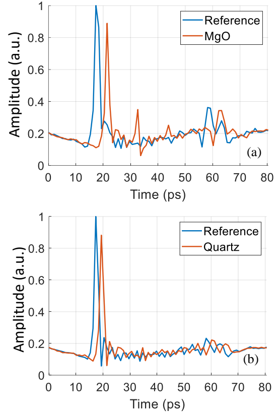
Fig. 8. The normalized amplitude of the complex envelope of the reconstructed temporal signals through the MgO and quartz samples: (a) MgO at x=6\text{mm} and z=5\text{mm} (orange curve) and the reference temporal signal corresponding to the same reconstructed coordinates (blue curve). (b) Quartz at x=-3\text{mm} and z=-3\text{mm} (orange curve) and the corresponding reference reconstructed temporal signal (blue curve).
