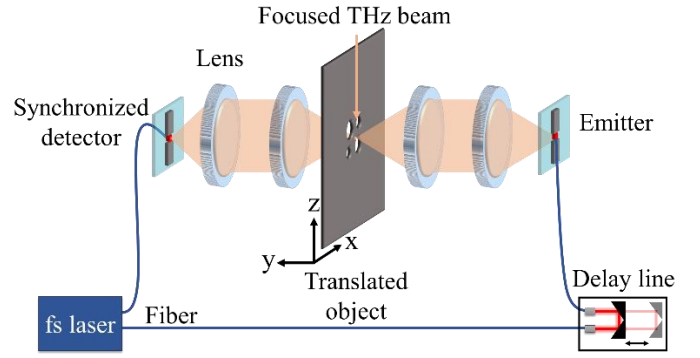
Fig. 2. Classical focused configuration of THz TDS. The imaged object is mechanically translated in the XOZ plane using a two-axis translation stage. The focal plane of the focused THz beam is achieved using four TPX lenses.
