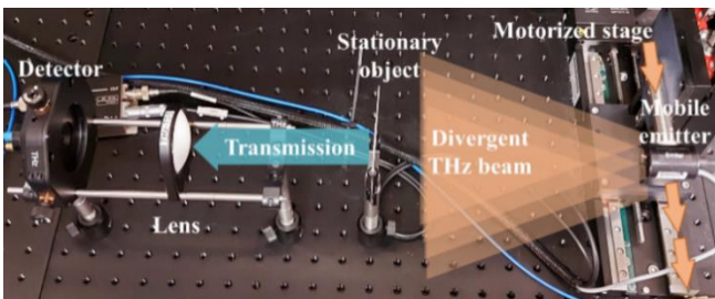
Fig. 6. Top view picture of the 3D SA-THz imaging system taken from top view, including a sketch of the divergent THz beam and propagation direction.
