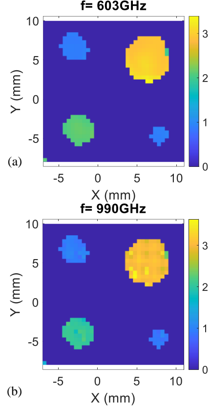
Fig. 10. 2D maps of the reconstructed refractive index of the dielectric samples within the imaged object at two different frequencies (a) at 603 GHz and (b) at 990 GHz. The 3D imaging performed beforehand is used to define the areas of interest, in which the refractive index reconstruction could be performed. The area of the metallic plate is set with a null refractive index for the visual aspect.
