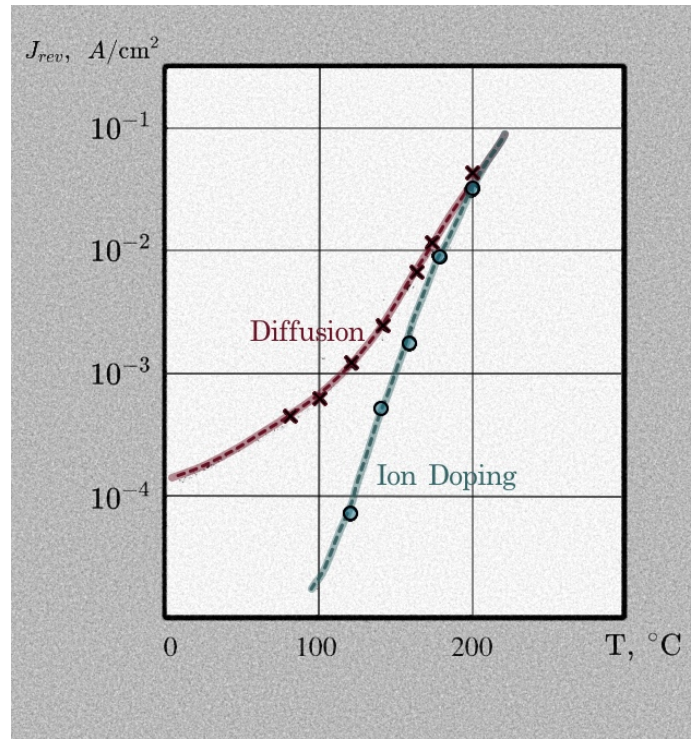
Figure 3: Dependence of insulating p-n junction reverse current density for MS #5: \times - with diffusion PCHs; \circ - with ion-alloyed PCHs.
