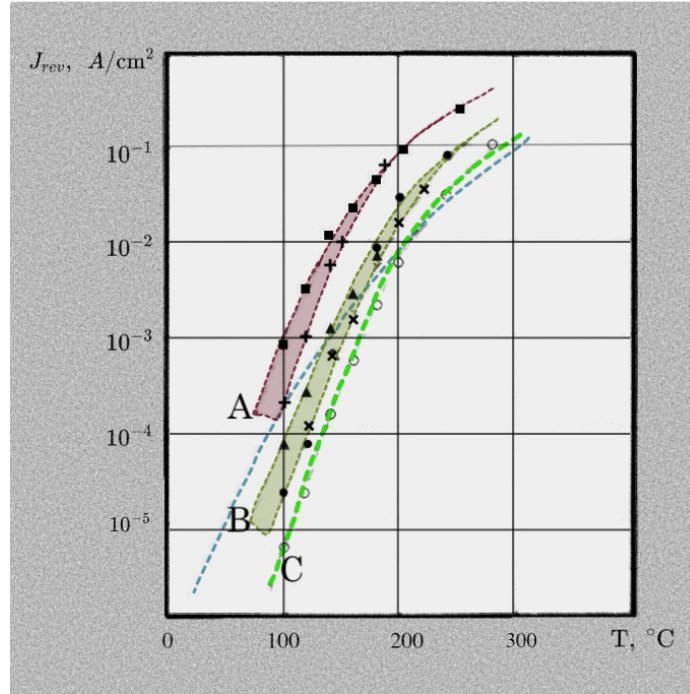
Figure 1: Temperature dependences of reverse current density of p-n junction isolating ion-alloyed and diffusion contact areas of the measuring circuit: \blacksquare - calculated from (3.10) \blacksquare - #1; \oplus - #2; \blacktriangle - #4; \bullet - #5; \otimes - #7; \circ - #10
