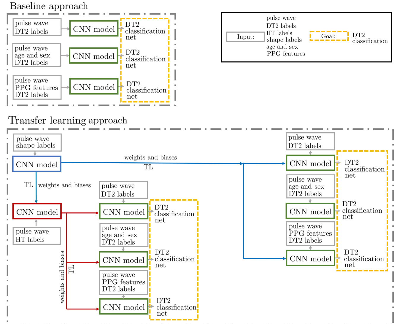
FIGURE 4. Overview of the proposed flow to assess the transfer learning efficacy in detecting diabetes. TL: transfer learning. HT: hypertension. DT2: type 2 diabetes. CNN: convolutional neural network.
