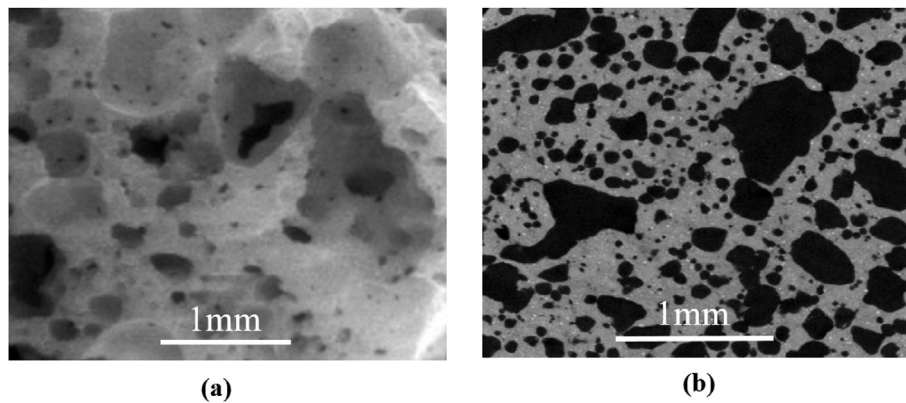
Fig. 4. (a) SEM image, (b) \mu CT slice image of HAP ceramic.
