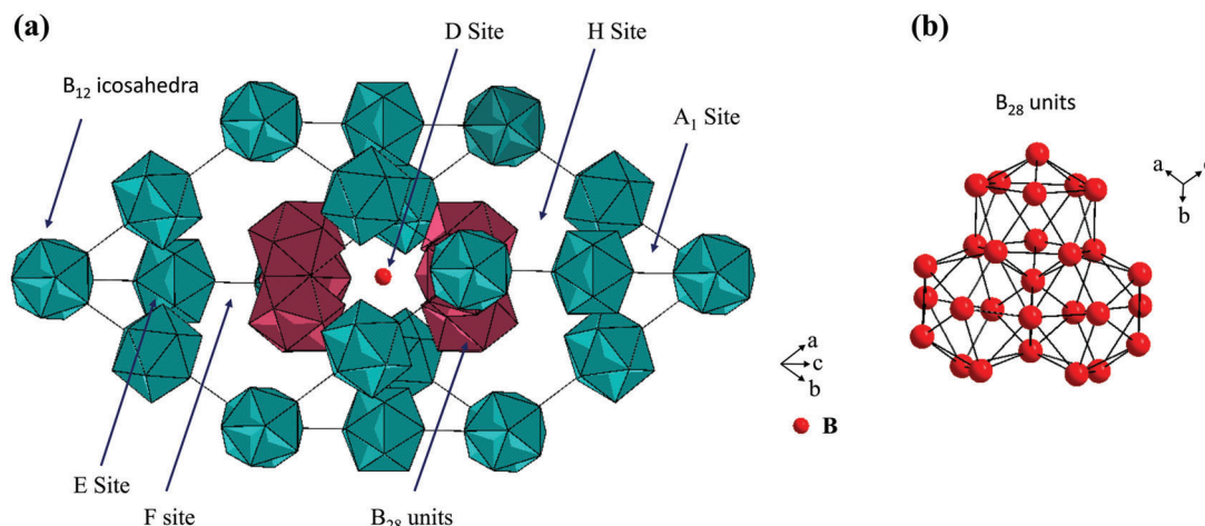
Figure 11. a) The crystal structure of \beta – boron, b) A detailed schematic of B_{28} units.
