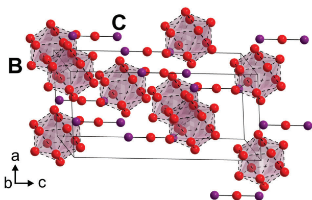
Figure 8. The crystal structure of B_{13}C_2 , a representative of boron carbides.
