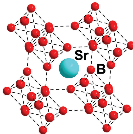
Figure 6. The crystal structure of SrB_6 , representative of hexaborides.
