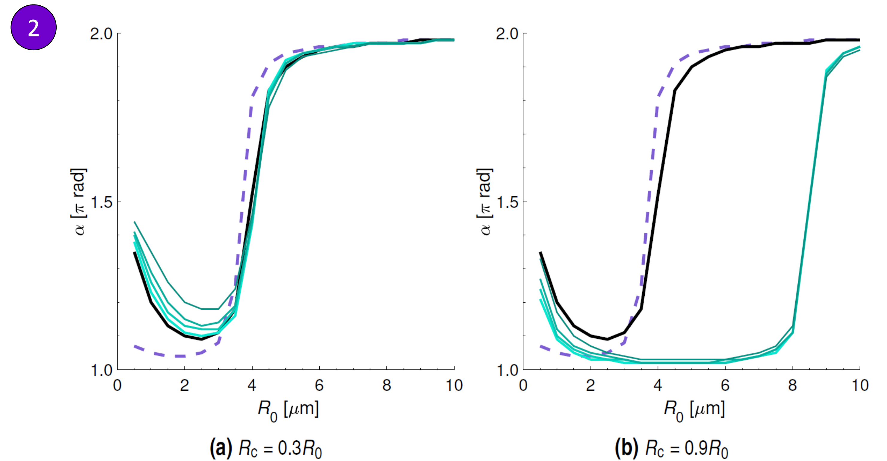
Pulsation phase with respect to incident sound field as a function of R_0 for a free gas bubble (—), an antibubble with no core (—), and antibubbles with core content having endoskeletal damping coefficients equal to 0.3 (—), 0.6 (—), 0.9 (—) and 2 (—).
