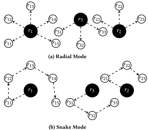
Figure 3: Exploration strategies.
