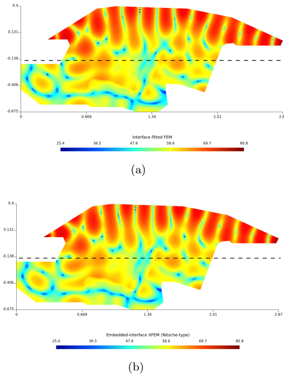
Figure 17: Snapshots of the numerical solution (pressure in dB) for (a) interface-fitted FEM with penalty-type formulation and (b) embedded interface X-FEM with Nitsche-type formulation.
