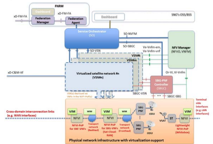
Figure II-1. Satellite-Terrestrial architecture
