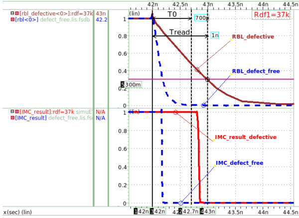
Figure 7. Waveforms of the sensitization sequence " \langle 1,0^N \text{ NOR}(1;0^N)/0^N/1 \rangle ", with N=127 " with df1 size set at 37kΩ.
