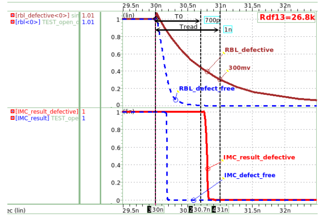
Figure 8. Waveforms of the sensitization sequence " \langle 1,0^N \text{ NOR}(1;0^N)/0^N/1 \rangle ", with N=127 " with df13 size set at 26.8kΩ.
