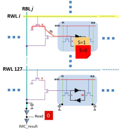
Figure 5. Faulty behavior of the bitcell in presence of df1
