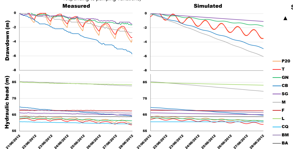
▼ Comparison of measured and simulated responses (drawdowns only for wells responding to pumping variations)
