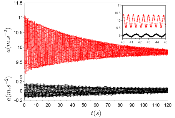
Figure 2: Radial (red) and orbital (black) accelerations measured by the accelerometer obtained with the experimental setup displayed in Fig. 1. Inset shows the temporal evolution of both accelerations between 40 s and 45 s. In order to have both curves on the same plot, orbital acceleration is shifted by a constant offset of 9 in the inset.
