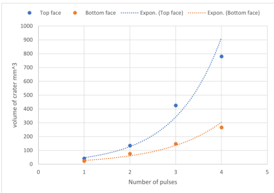
Fig. 7. Volume of crater as function of number of pulses for dry sandstone (voltage fixed at 90 kV, electric field = 4.5 kV/mm)
