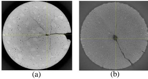
Fig. 8. Selected cross-sectional image X–Y slices of the tested specimens. (a) concrete (b) sandstone
