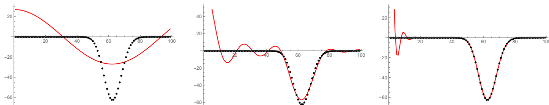
Figure 12: The sequence s_g for z = -10^{-8} in local \mathbb{P}^2 is represented in black dots and compared to the expected oscillatory behavior (362) (red line), where we include only a finite number of terms in the sum. In the first figure, we include only m = 0 , in the second m = 0, 1, 2 , and in the third m = 0, 1, \dots, 8 .
