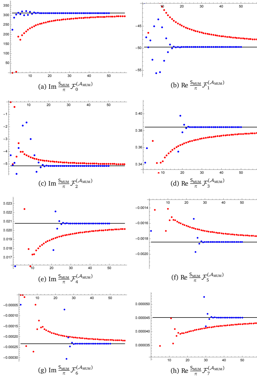
Figure 15: Comparison between auxiliary sequences (similar to (376), red dots) that asymptote to \frac{S_{\text{MUM}}}{\pi} \mathcal{F}_g^{(\text{MUM})} ( g = 0, 1, \dots, 7 ) constructed from evaluation of \mathcal{F}_g(X^1, P_0) up to g = 61 with S_{\text{MUM}} = -\chi , their Richardson transformations (8-th order, blue dots), and the prediction from the 1-instanton formula (278) (black line) for the X^0 instanton sector in the case of the quintic.
