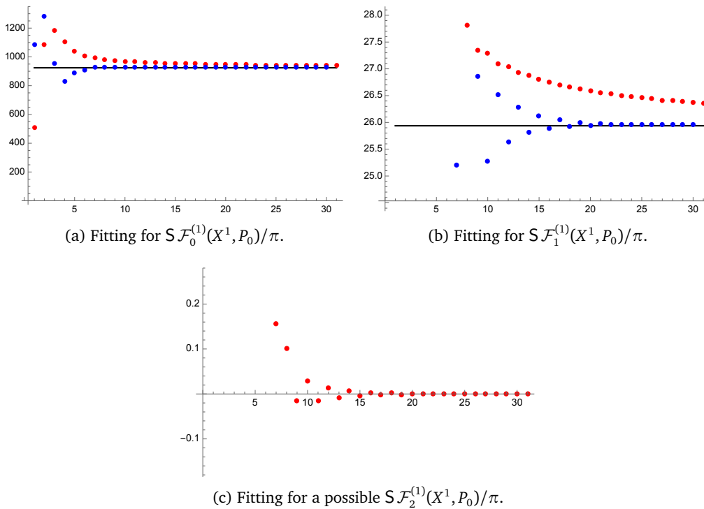
Figure 13: Comparison between auxiliary sequences (367), (368), (369) (red dots) which asymptote to S_1 \mathcal{F}_{0,1,2}^{(1)}(X^1, P_0)/\pi with S_1 = n_{0,1} , their Richardson transforms (1st-order, blue dots), and the prediction (366) (black lines) for the example of the X_{2,2,2,2}(1^8) model at z = (1 - 10^{-6})\mu .
