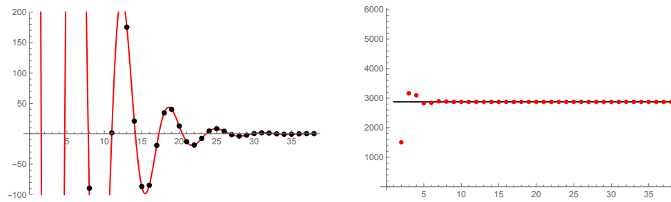
Figure 11: On the left, the sequence s_g (black dots) as compared to the expected oscillatory behavior (359) (red line), when z = 10^{-5} . On the right, the sequence s_g minus its oscillatory part (red dots) and the prediction 2875 (black line).
