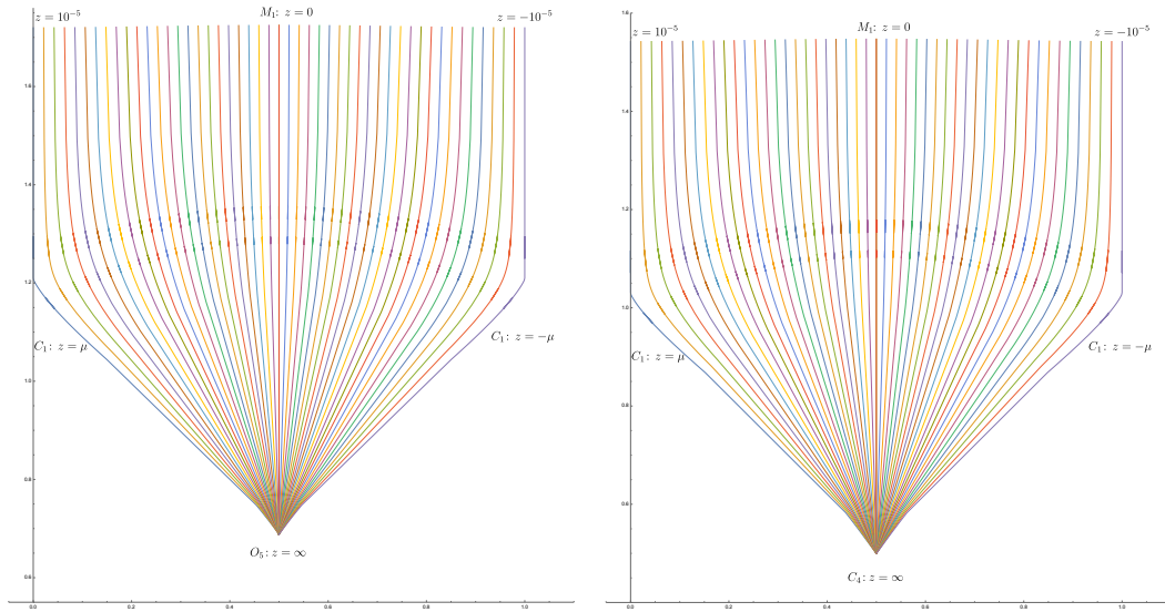
Figure 1: The values of t = X^1/X^0 over the cut z -plane for the model X_5(1^5) with an O-point of unipotent l = 5 at z = \infty (left) and the model X_{4,2}(1^6) with a C-point of unipotent l = 4 at z = \infty (right). The plots depict the t image of rays in the z -plane emanating from the semi-circle with radius 10^{-5} in radial direction towards infinity. \text{Im } t \rightarrow \infty corresponds to z = 0 .
