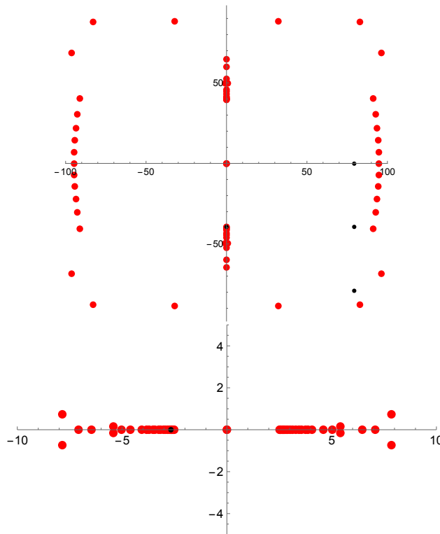
Figure 9: The location of the poles of the Padé approximant to \widehat{\mathcal{F}}^{\text{hol}} evaluated to order g = 64 at the point z = 10^{-2}\mu on the left, and z = \frac{5}{6}\mu on the right. The black dots on the left give the positions of the periods \Re(mX^0 + nX^1) , (m, n) = (1, 0), (0, 1), (1, 1), (2, 1) , while the black dot on the right gives the position of \Re P_0 .
