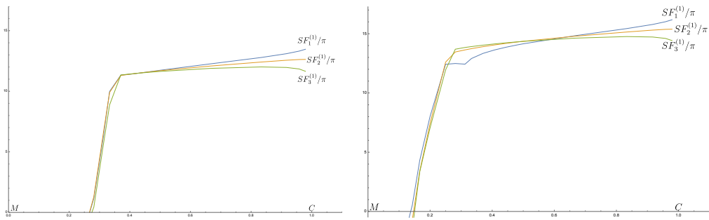
Figure 14: The significant digits of the asymptotic estimates for 1 instanton genus 1, 2, 3 contributions without (left) and with (right) constant map subtraction for the quintic X_5(1^5) to g = 64 .
