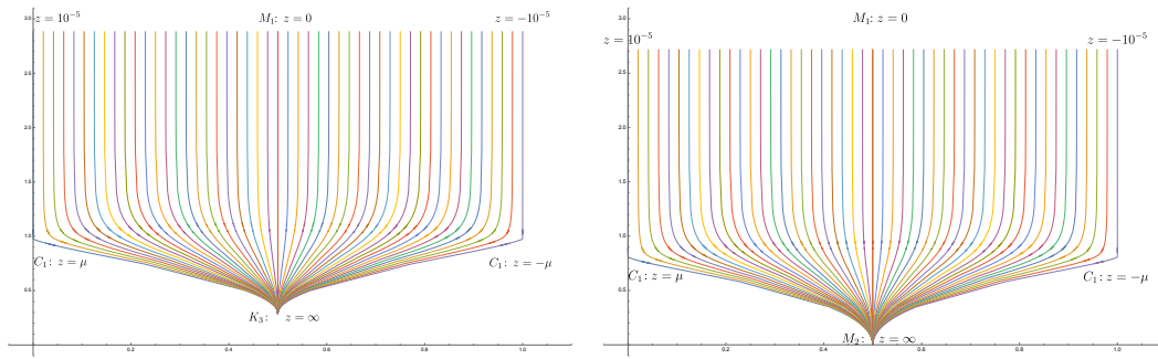
Figure 2: The values of t = X^1/X^0 over the cut z -plane, plotted as explained in the caption of Figure 1, for the model X_{33}(1^6) with a K-point of unipotentcy l = 3 at z = \infty (left) and the model X_{2222}(1^9) with an M-point of unipotentcy l = 2 at z = \infty (right).
