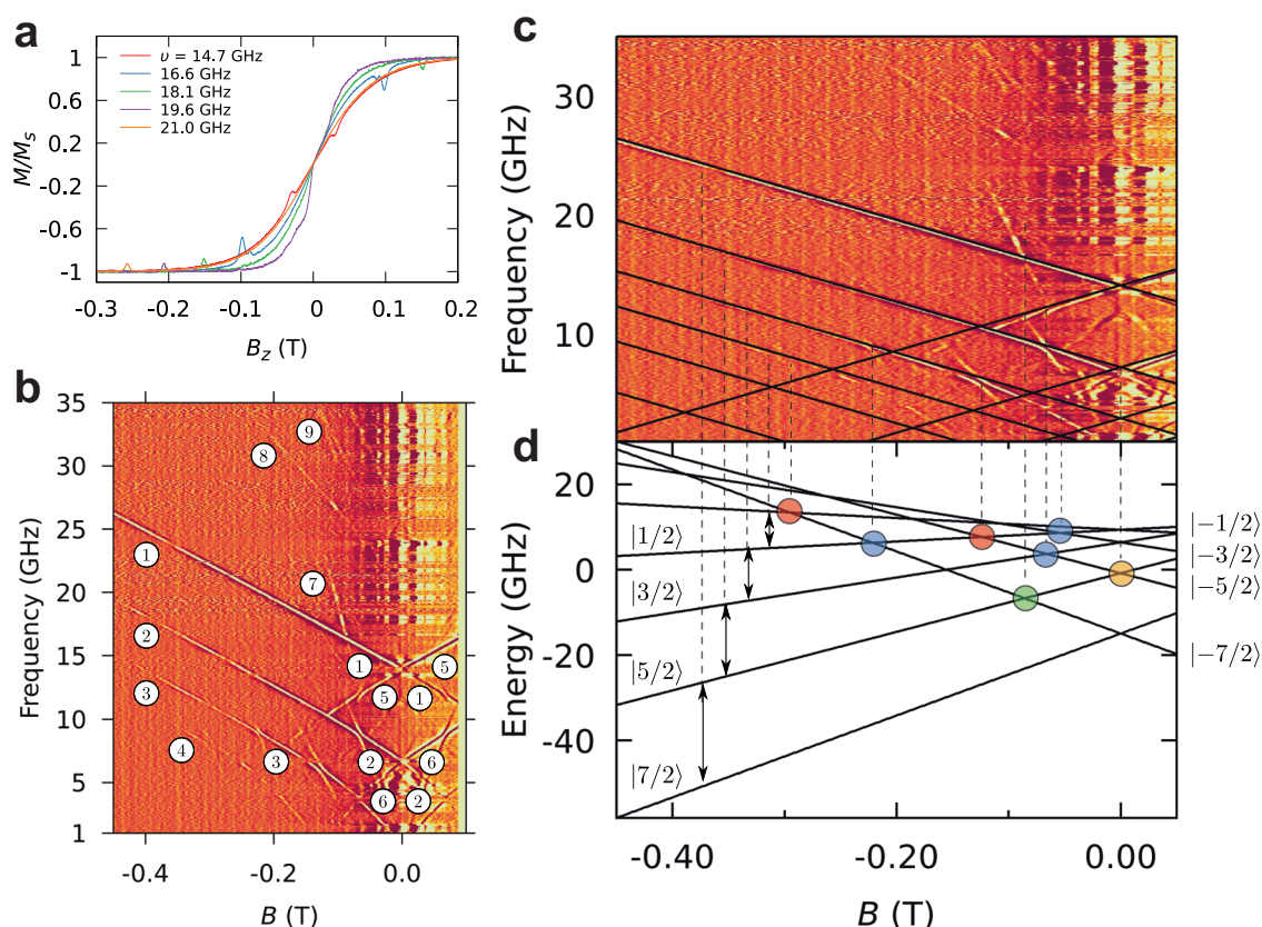
Fig. 3 | \mu SQUID loops EPR. a Magnetisation curves as a function of the frequency of the RF source obtained while sweeping the magnetic field with a fixed sweeping rate of 8 mT/s and by applying pulses of 40 \mu s width and 300 \mu s period. b Resonance maps obtained by sweeping along the easy axis with a constant sweeping rate of 8 mT/s and applying RF pulses with 40- \mu s width every 300 \mu s. The labels correspond to (m, m') transitions (see the main text). c Linear fit of the resonance map by
