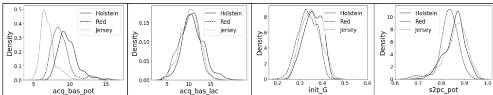
Figure 4. Posterior distributions of the genetic-scale parameters between breeds.
