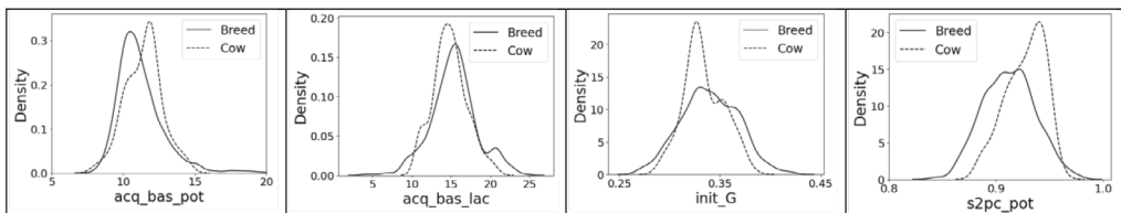
Figure 3. Posterior distributions of the genetic-scale parameters for a breed and an example of one individual of that breed.
