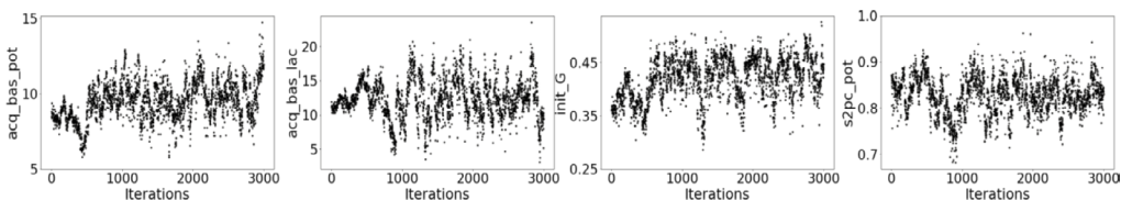
Figure 2. Example of the Markov chains of genetic-scale parameters.
