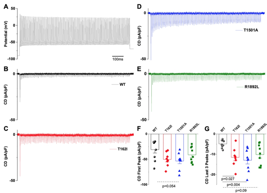
Figure 3. Action sodium currents recorded using as voltage stimulus an action potential discharge of a GABAergic fast spiking neuron, shown in panel (A). Action \text{Na}^+ currents for hNav1.1-WT (B), hNav1.1-T162I (C), hNav1.1-T1501A (D), hNav1.1-R1892L (E); traces are presented as mean current densities (CD), for clarity error bars are not shown. (F) Comparison of the peak current density of the first action current. (G) Comparison of the peak current density at the end of the discharge (mean of the 3 last action currents).
