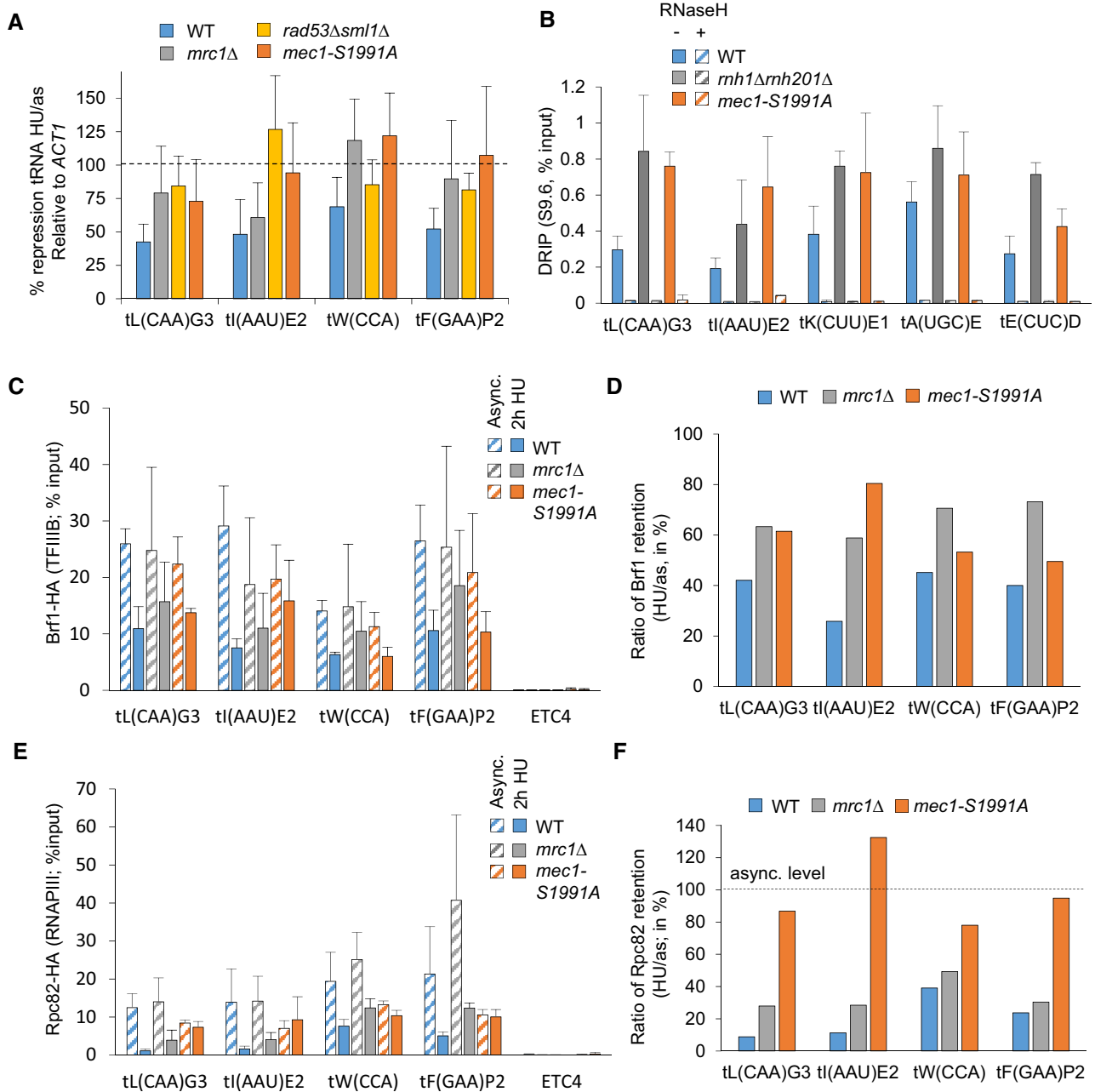
Figure 4. Mec1-S1991 phosphorylation limits RNAPIII transcription on HU.
